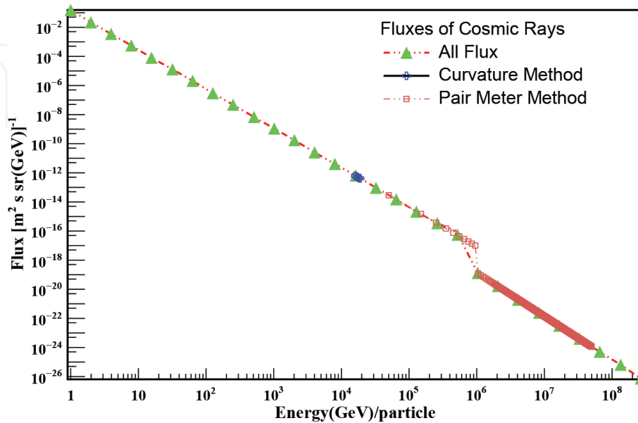
Figure 7. Primary cosmic ray flux ( \phi \approx KE^{-\alpha} , where \alpha \approx 2.7 and for KNEE (3PeV) \alpha: 2.7 \rightarrow 3 ) versus energy of primary particle, and limited range for ICAL to cover the spectrum using magnetic field and pair meter technique.
