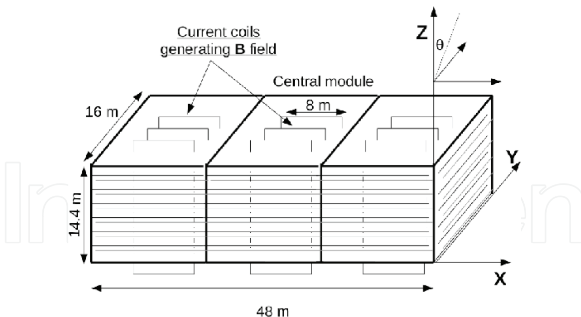
Figure 1. Schematic view of three modules for the proposed INO-ICAL detector.
