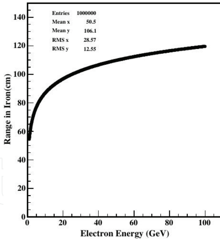
Figure 5. Energy of the electron and its corresponding penetrating range in the iron plates.
