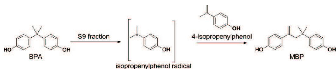
Figure 5. BPA metabolic activation through formation of the potent estrogenic metabolite MBP [61].
