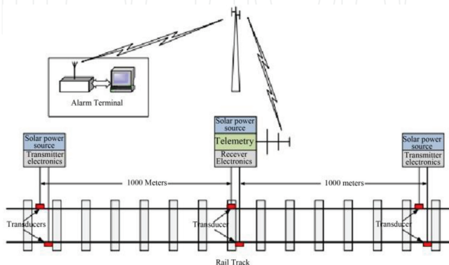
Figure 5. Monitoring system on freight line in South Africa [66].
