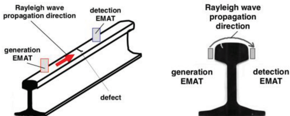
Figure 4. Rail cracks detection using EMAT [59].
