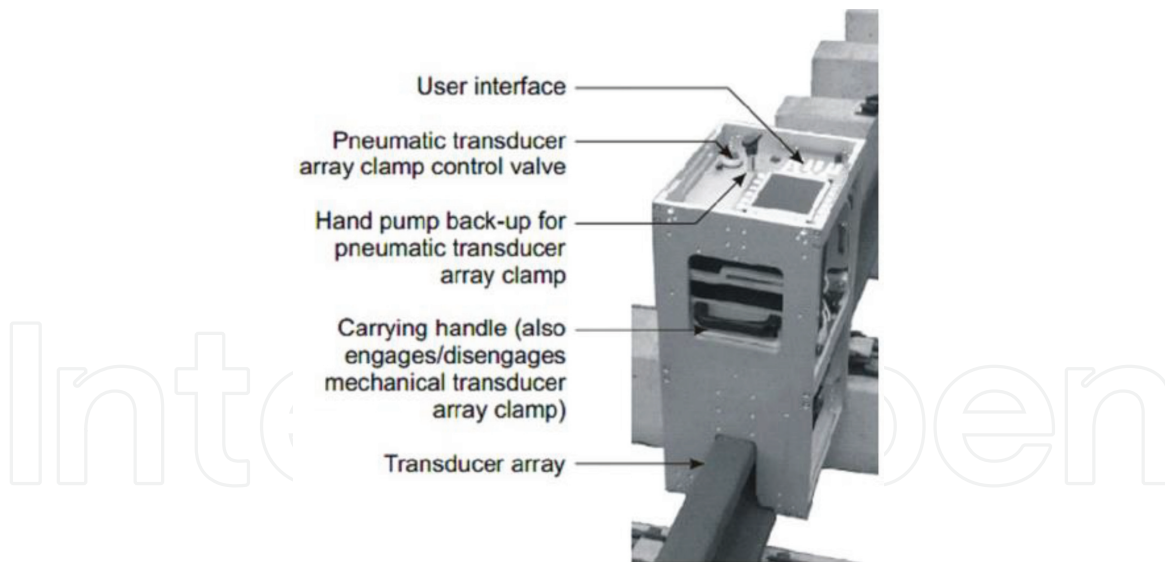
Figure 6. G-type scan guided wave in inspection device in UK [67].
