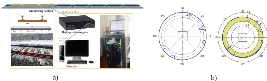
Figure 3. High-speed train wheel defect detection using online FBG-based system [36]. (a) System configuration. (b) Detection results (left—online detection; right—offline inspection).
