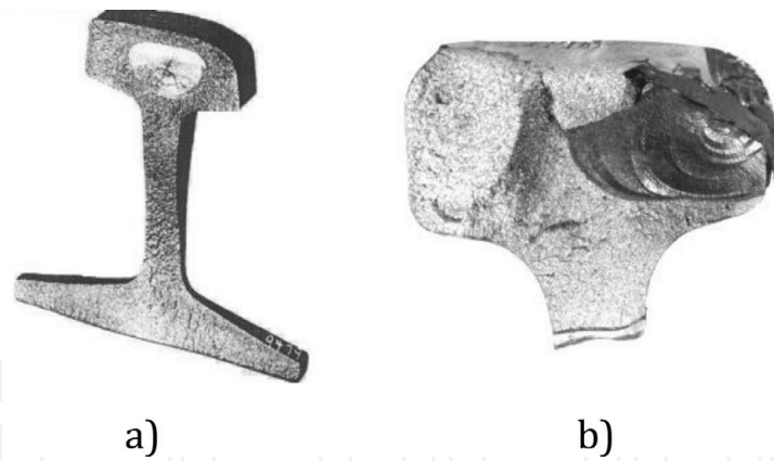
Figure 1. Transverse defect and detail fracture [15]. (a) Transverse defect. (b) Detail fracture.
