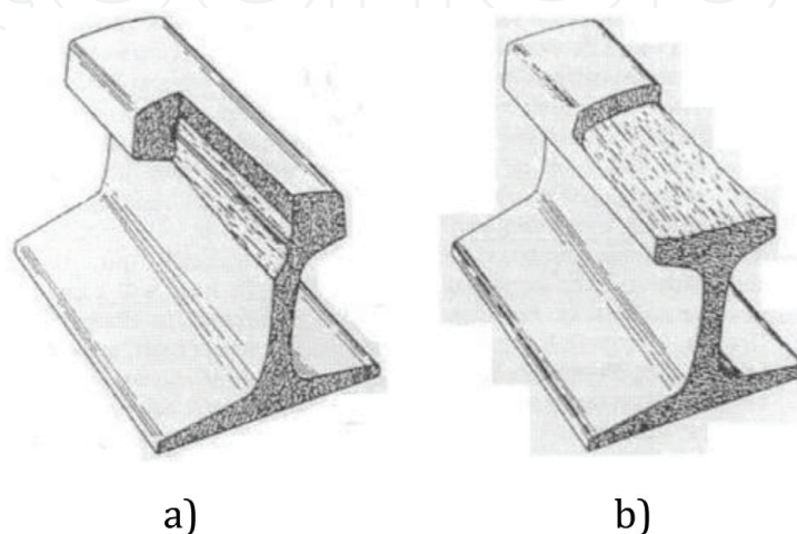
Figure 2. Split head [16]. (a) Vertical split head. (b) Horizontal split head.
