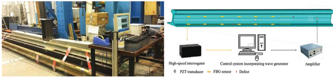
Figure 8. Schematic set-up of the FBG-PZT monitoring system [79].
