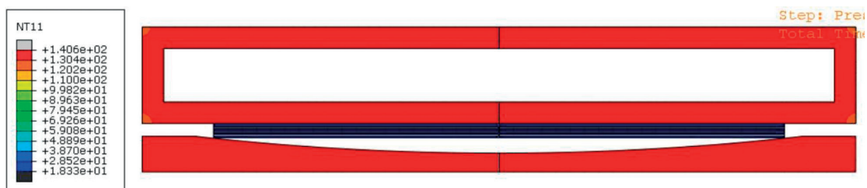
Figure 11. Nodal temperature results at t = 120 s (bladder completely heated up).
