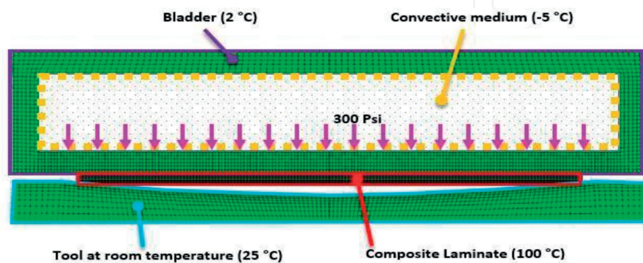
Figure 7. Initial temperatures for each part.
