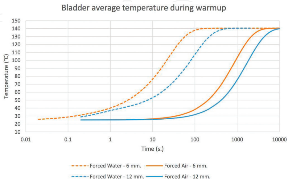
Figure 22. Bladder temperature history.
