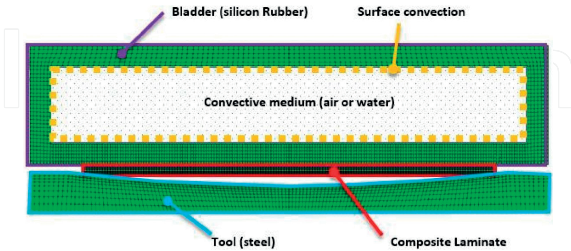
Figure 5. Assigned materials for each component.
