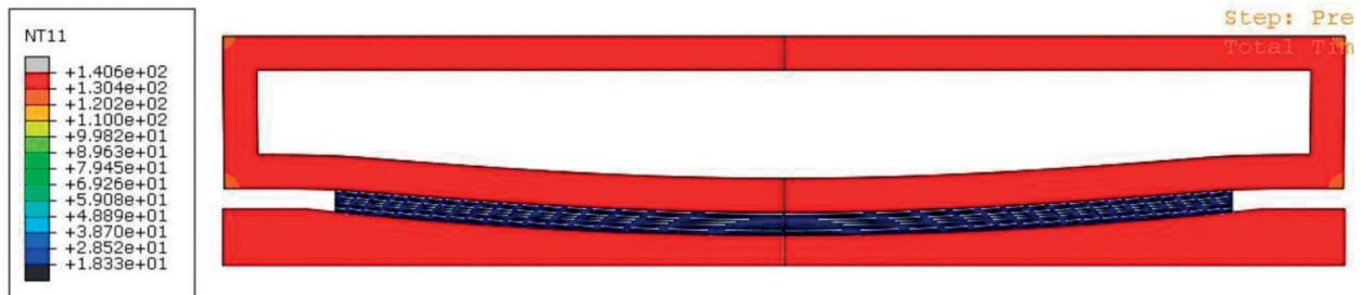
Figure 12. Expanded bladder due to applied pressure of 300 psi (the composite plate and tool are in contact).
