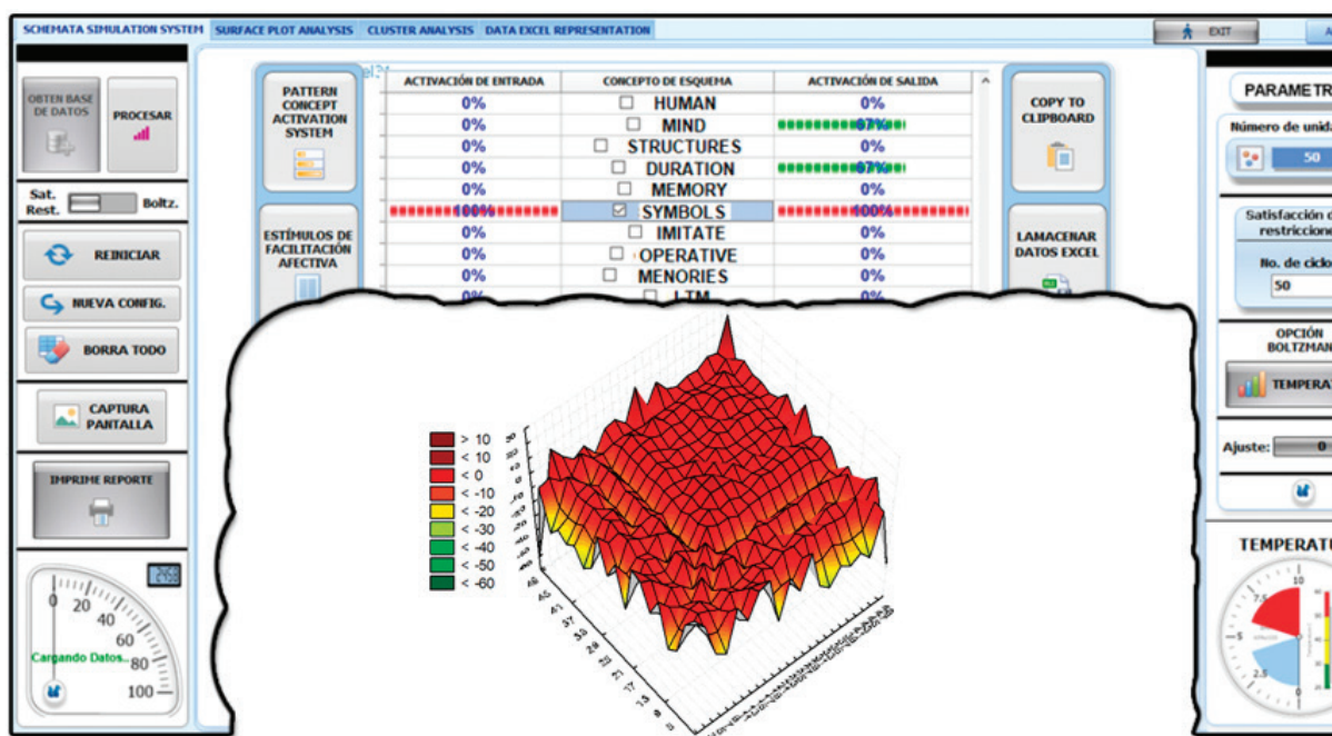
Figure 6. User interface for modeling schema-based behavior, and a surface plot of its underlying weight association matrix (bottom center).
