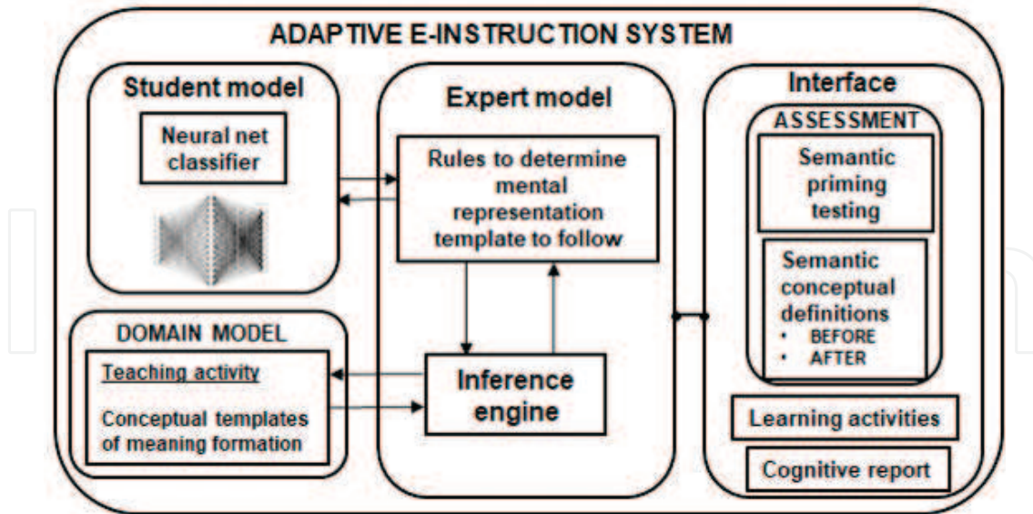
Figure 9. Proposal for adaptive instruction/assessment instruction.
