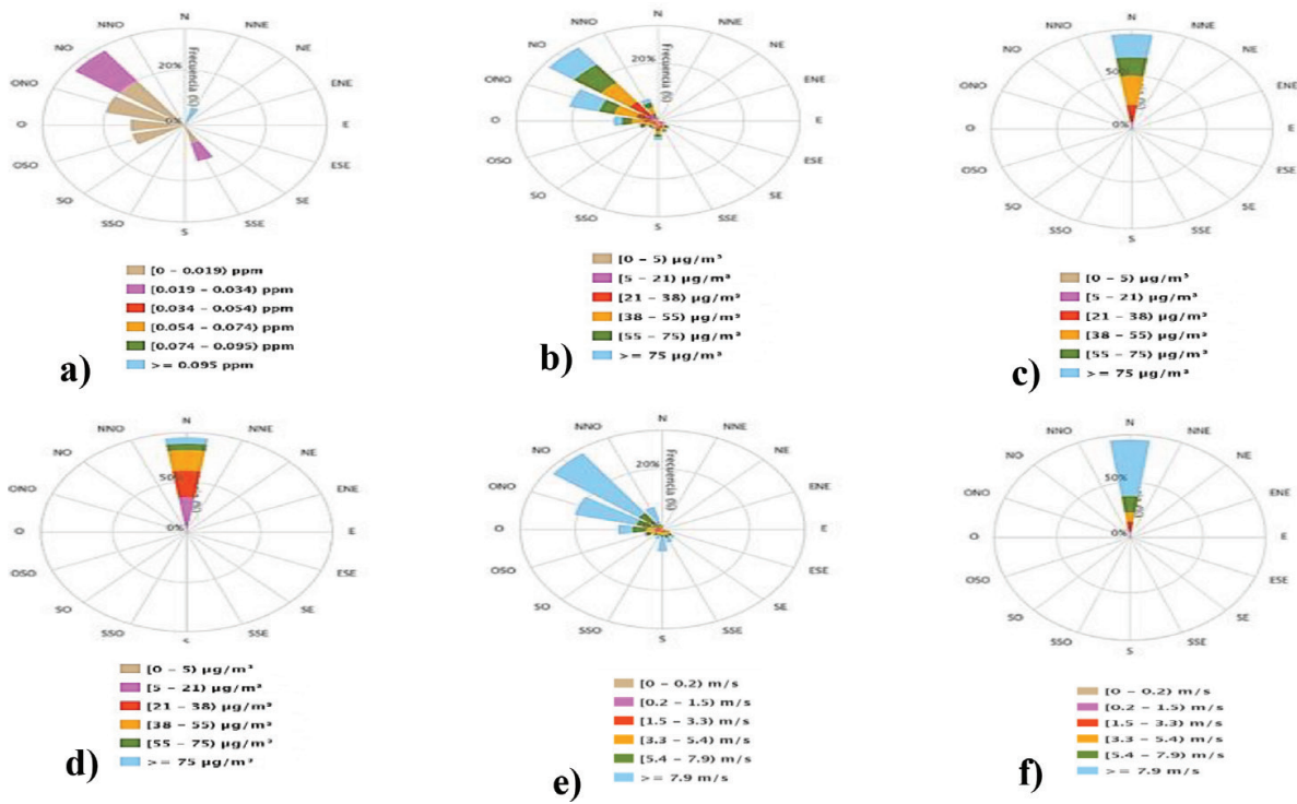
Figure 7. Criteria air pollutants and meteorological conditions for site V (Apodaca) during the study period: (a) \text{O}_3 dry season, (b) \text{PM}_{10} dry season, (c) \text{PM}_{10} rainy and cold fronts seasons, (d) \text{PM}_{2.5} rainy and cold fronts seasons, (e) wind dry season, (f) wind rainy and cold fronts seasons.
