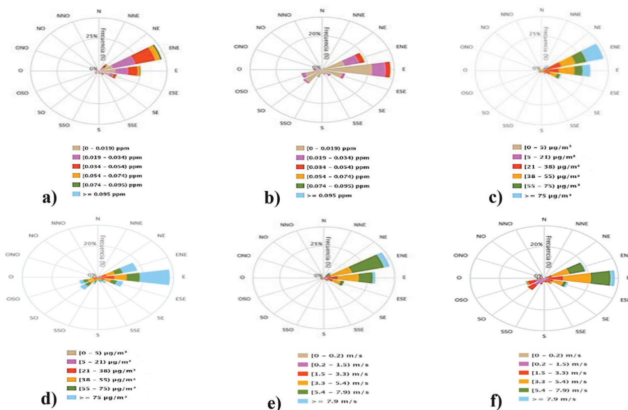
Figure 10. Criteria air pollutants and meteorological conditions for Site VIII (San Pedro) during the study period: (a) O 3 dry and rainy seasons, (b) O 3 cold fronts season, (c) PM 10 dry and rainy seasons, (d) PM 10 cold fronts season, (e) wind dry and rainy seasons, (f) wind cold fronts season.
