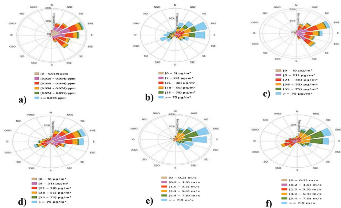
Figure 8. Criteria air pollutants and meteorological conditions for site VI (Obispado) during the study period: (a) \text{O}_3 dry, rainy and cold fronts seasons, (b) \text{PM}_{10} dry, rainy and cold fronts seasons, (c) \text{PM}_{2.5} dry and rainy seasons, (d) \text{PM}_{2.5} cold fronts season, (e) wind dry and rainy season, (f) wind cold fronts season.
