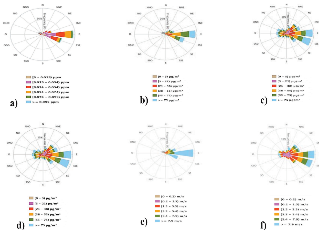
Figure 3. Criteria air pollutants and meteorological conditions for site I (Escobedo) during the study period: (a) O 3 dry season, (b) PM 10 dry, and rainy seasons, (c) PM 10 cold fronts season, (d) PM 2.5 cold fronts season, (e) wind dry and rainy season, (f) wind cold fronts season.
