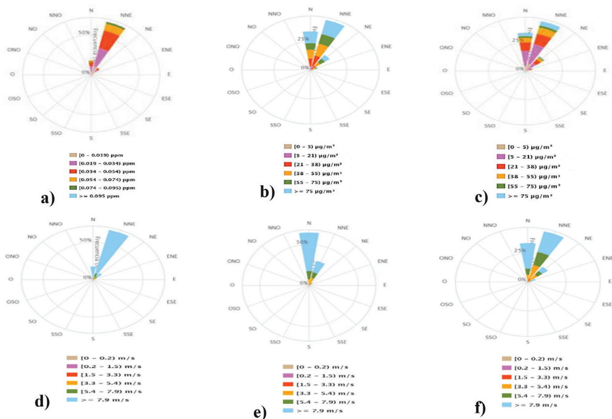
Figure 11. Criteria air pollutants and meteorological conditions for site IX (La Pastora) during the study period: (a) O 3 dry, rainy and cold fronts seasons, (b) PM 10 dry, rainy, and cold fronts seasons, (c) PM 2.5 dry, rainy, and cold fronts seasons, (d) wind dry season, (e) wind rainy season, (f) wind cold fronts season.
