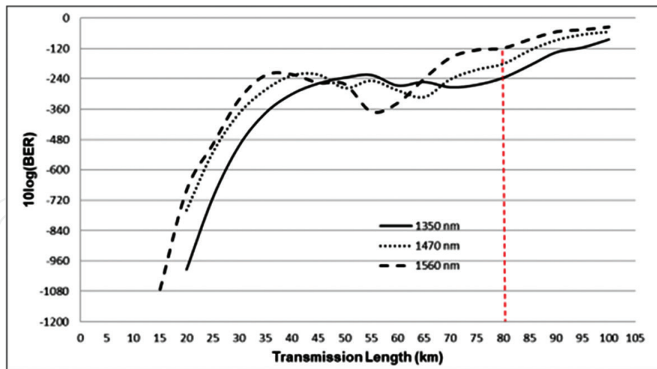
Figure 19. BER value to transmission length.
