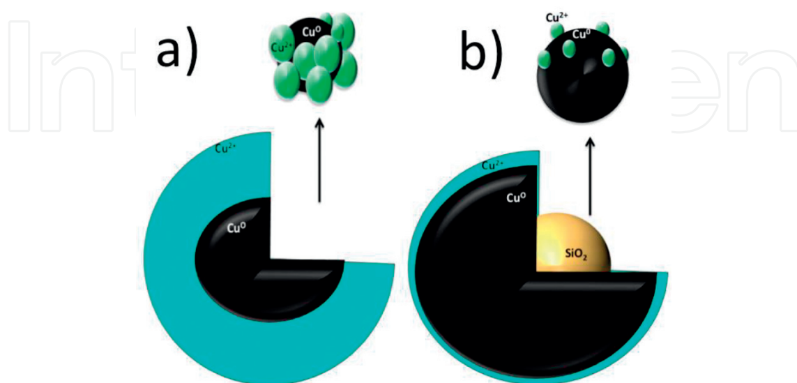
Figure 3. (a) Chi/Cu/CuO core-shell nanoparticle (b) Chi/Cu/CuO@SiO 2 core-shell nanoparticle.
