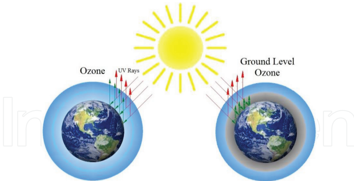
Figure 1. Ozone & ground level ozone and greenhouse effect.
