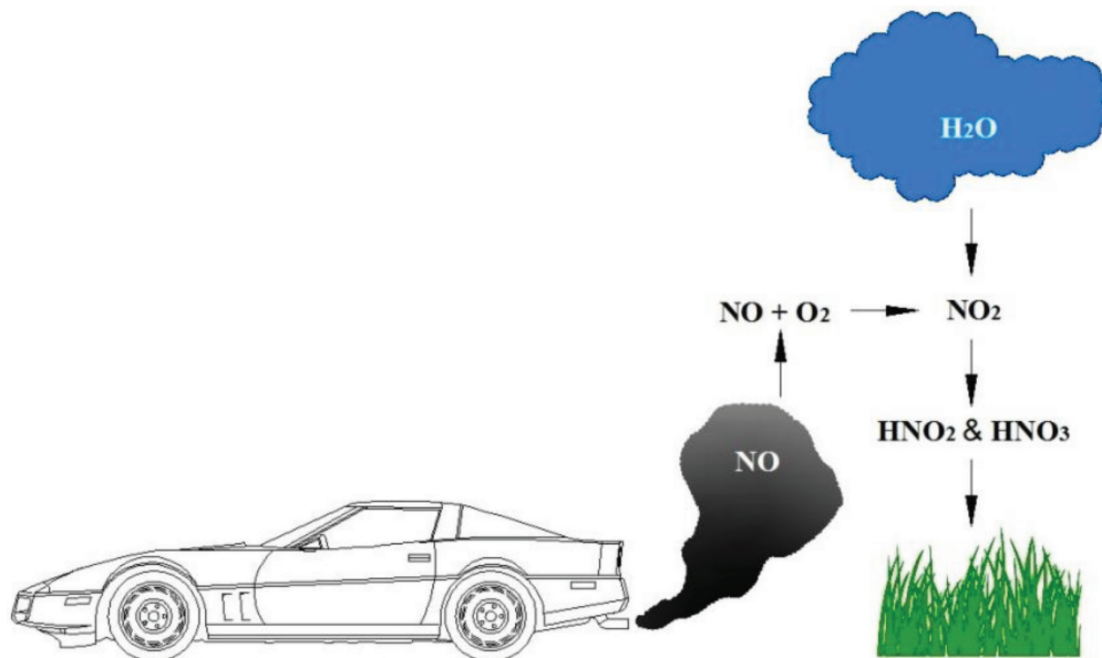
Figure 2. The formation of acid rains.
