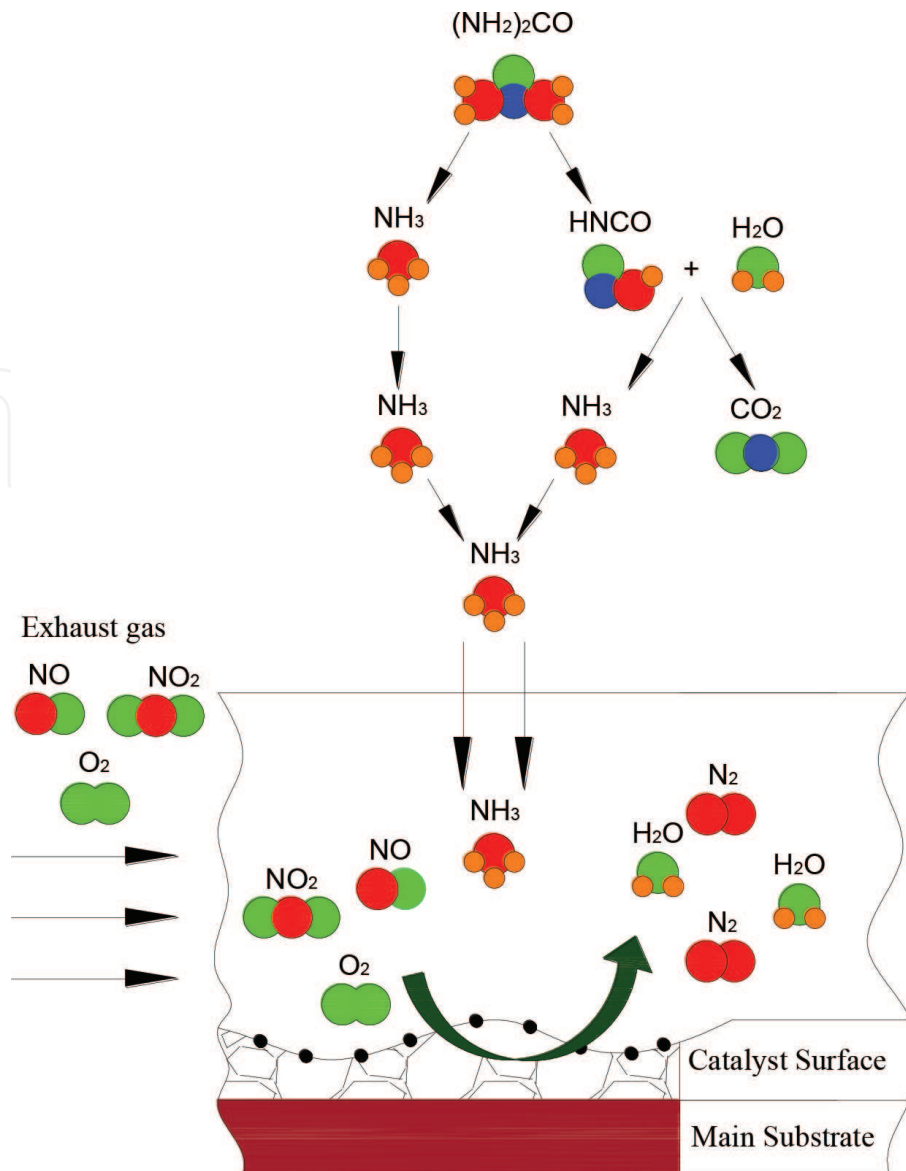
Figure 5. NO x conversion reactions in NH 3 -SCR.
