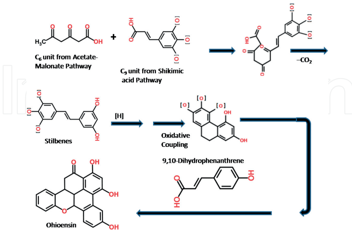
Figure 2. Synthesis of Ohioensins.
