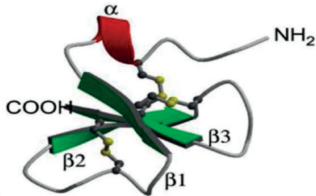
Figure 1. Secondary structure of HBD-2 that consists of an N-terminal region linked to an alpha helix, three \beta -strands arranged in an antiparallel sheet and a C-terminal region [41].
