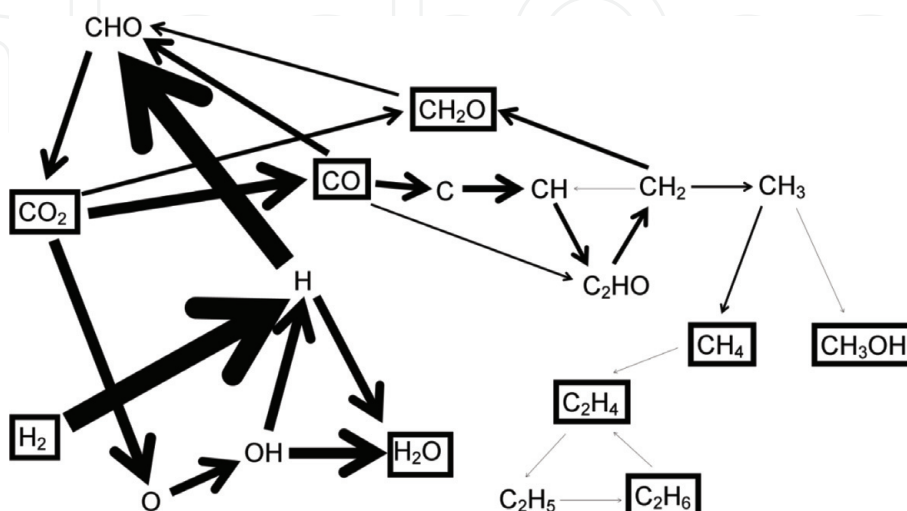
Figure 6. Dominant reaction pathways for the conversion of \text{CO}_2 and \text{H}_2 into various products, in a 50/50 \text{CO}_2/\text{H}_2 DBD plasma, as obtained from the model in [75]. The thickness of the arrow lines corresponds to the rates of the net reactions. The stable molecules are indicated with black rectangles. Reproduced from [75] with permission.
