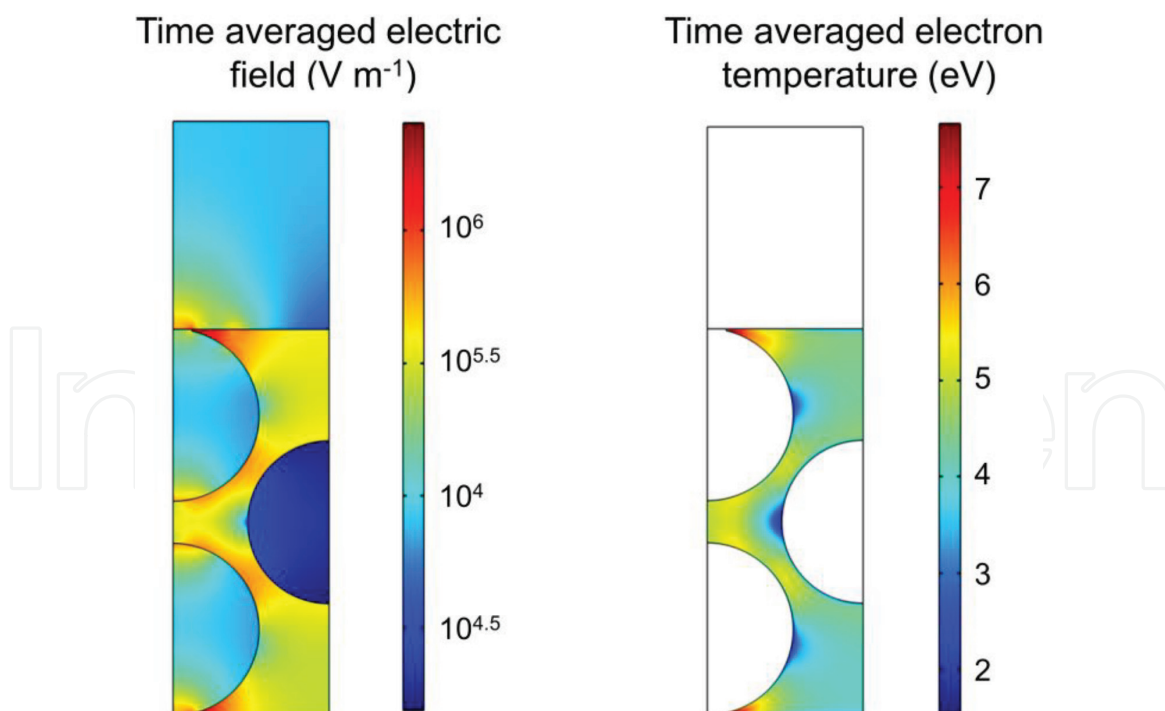
Figure 8. Calculated time-averaged 2D profiles of the electric field and electron temperature in a packed bed DBD reactor, at a peak-to-peak voltage of 4 kV and a frequency of 23.5 kHz, as obtained from the model in [94]. Adopted from [94] with permission.
