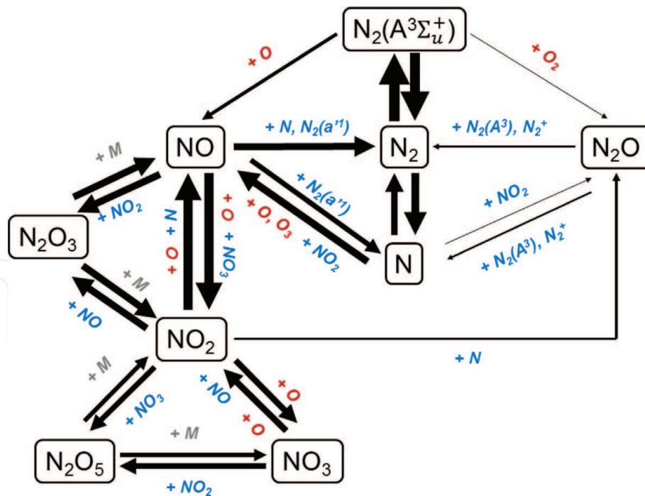
Figure 7. Dominant reaction pathways leading to NO x formation in a CO 2 /N 2 DBD plasma, as obtained from the model in [77]. See details in the text. The thickness of the arrow lines corresponds to the time-integrated reaction rates, indicating the importance of the reactions. Adopted from [77] with permission.
