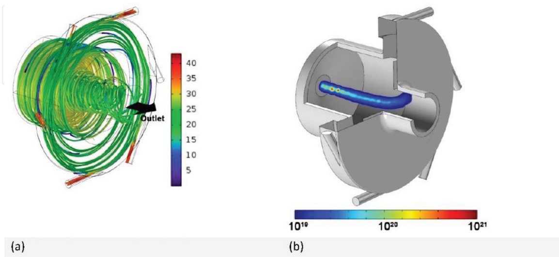
Figure 11. Calculated steady-state gas flow stream lines (a) and electron density at a time of 5.3 ms, when the arc is stabilized in the center (b), for a reverse vortex flow GA plasma reactor at an arc current of 240 mA, as obtained from the model in [87].
