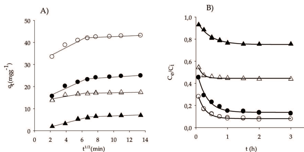
Figure 1. (A) IPD plots for MSM kinetic sorption on ultisol (▲) and andisol (Δ); and DI kinetic sorption on ultisol (●) and ndisol (O); (B) TSNE model plot for MSM sorption on ultisol (▲) and andisol (Δ) and DI sorption on ultisol (●) and andisol (O) [7, 9].
