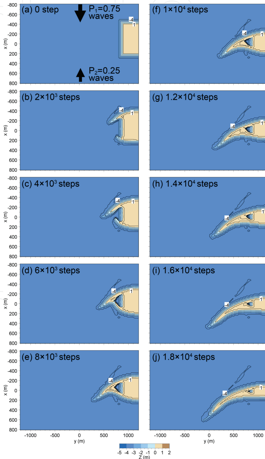
Figure 9. Extension of cusped foreland in Case 3.
