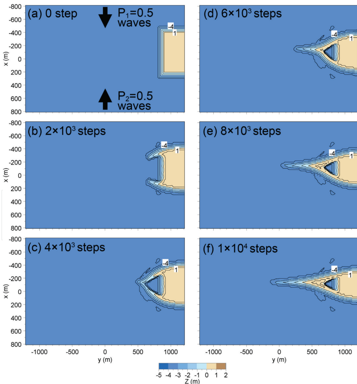
Figure 8. Extension of cusped foreland in Case 2.
