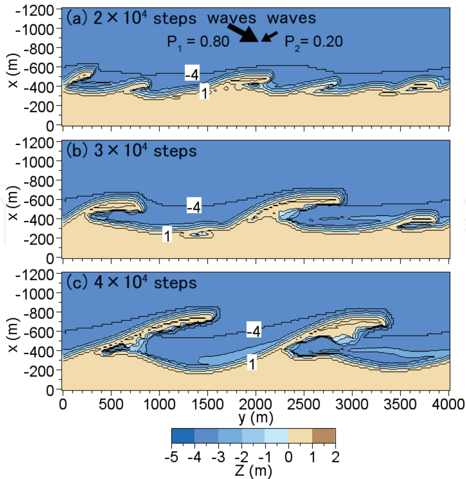
Figure 19. Formation of cusped forelands when waves were obliquely incident at angles of \pm 60^\circ with probability of 0.80:0.20 [5].
