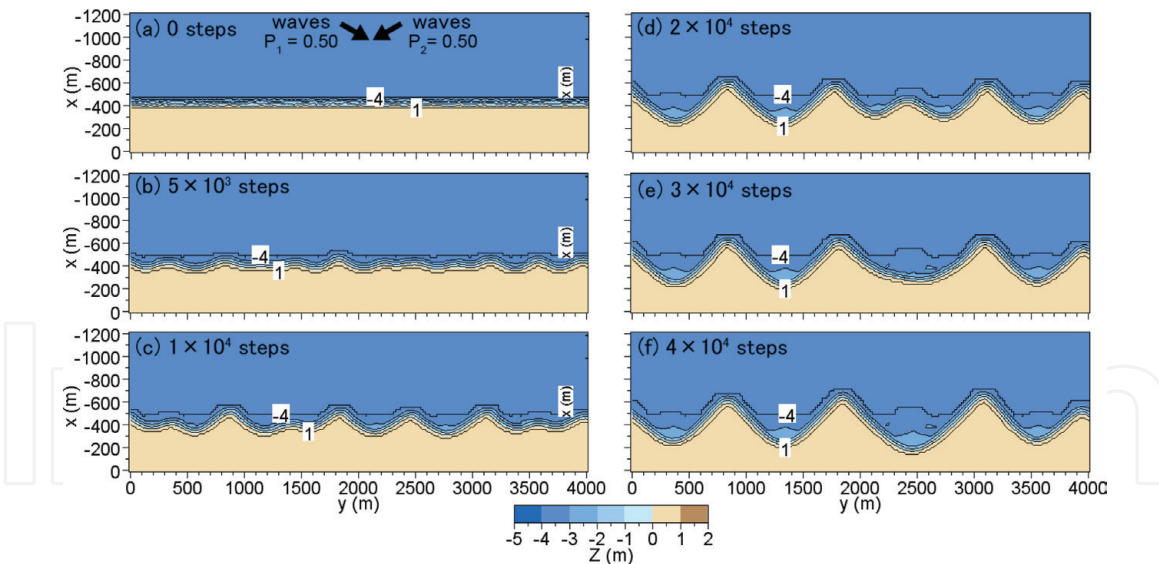
Figure 13. Formation of cusate forelands when waves were obliquely incident at angles of \pm 60^\circ with probability of 0.50:0.50 [4, 5].
