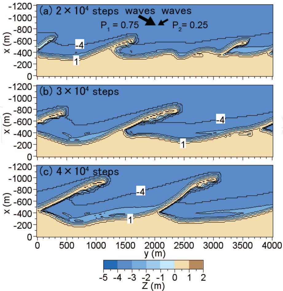
Figure 18. Formation of cuspate forelands when waves were obliquely incident at angles of \pm 60^\circ with probability of 0.75:0.25 [5].
