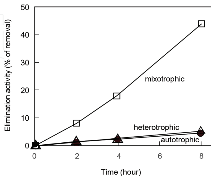
Figure 8. Elimination of Cs-137 from the medium by G. sulphuraria . Cells were incubated without 25 mM glucose under light condition (autotrophic condition, closed circle), with 25 mM glucose under light condition (mixotrophic condition, open square), or with 25 mM glucose under dark condition (heterotrophic condition, open triangle).
