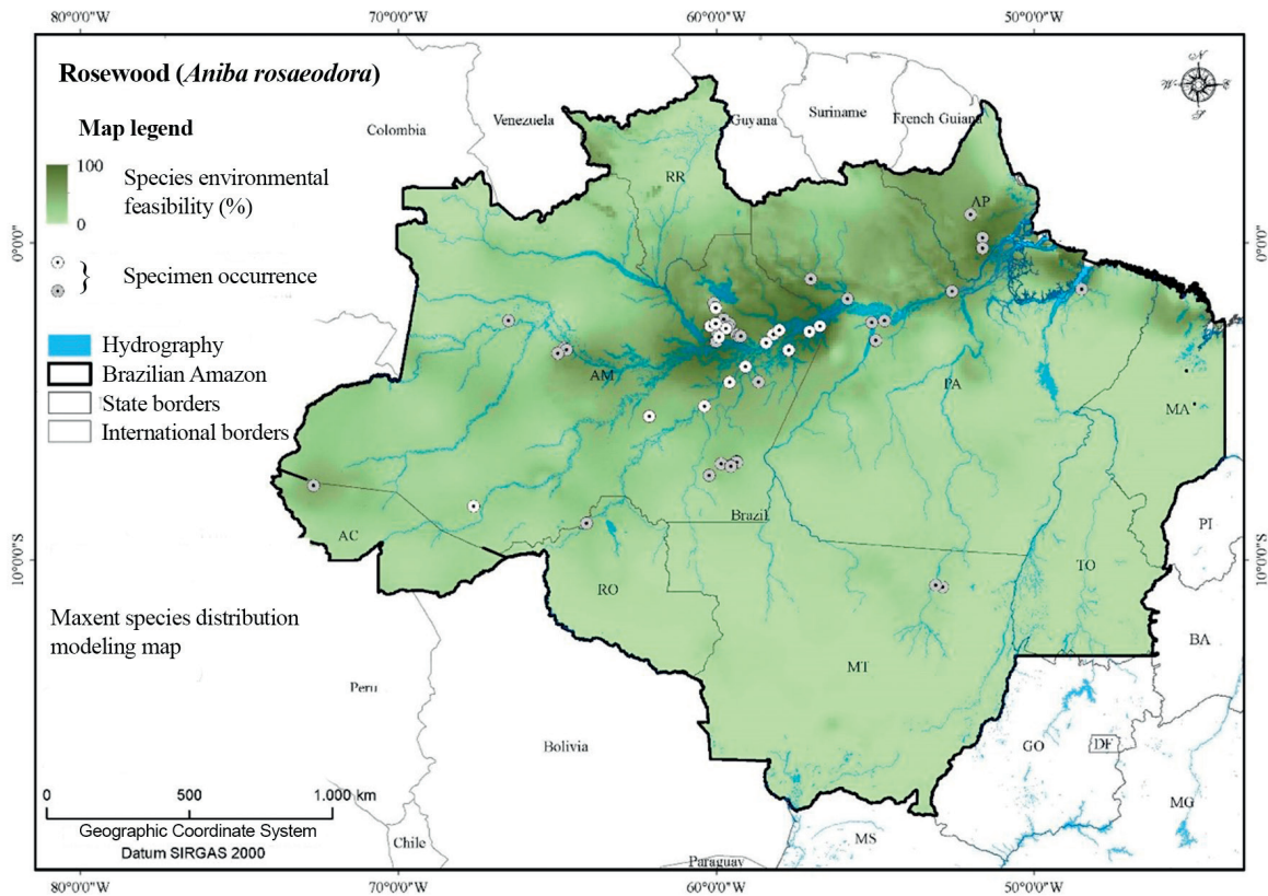
Figure 5. Geographic distribution for rosewood ( Aniba rosaeodora ) in the Brazilian Amazon [21].
