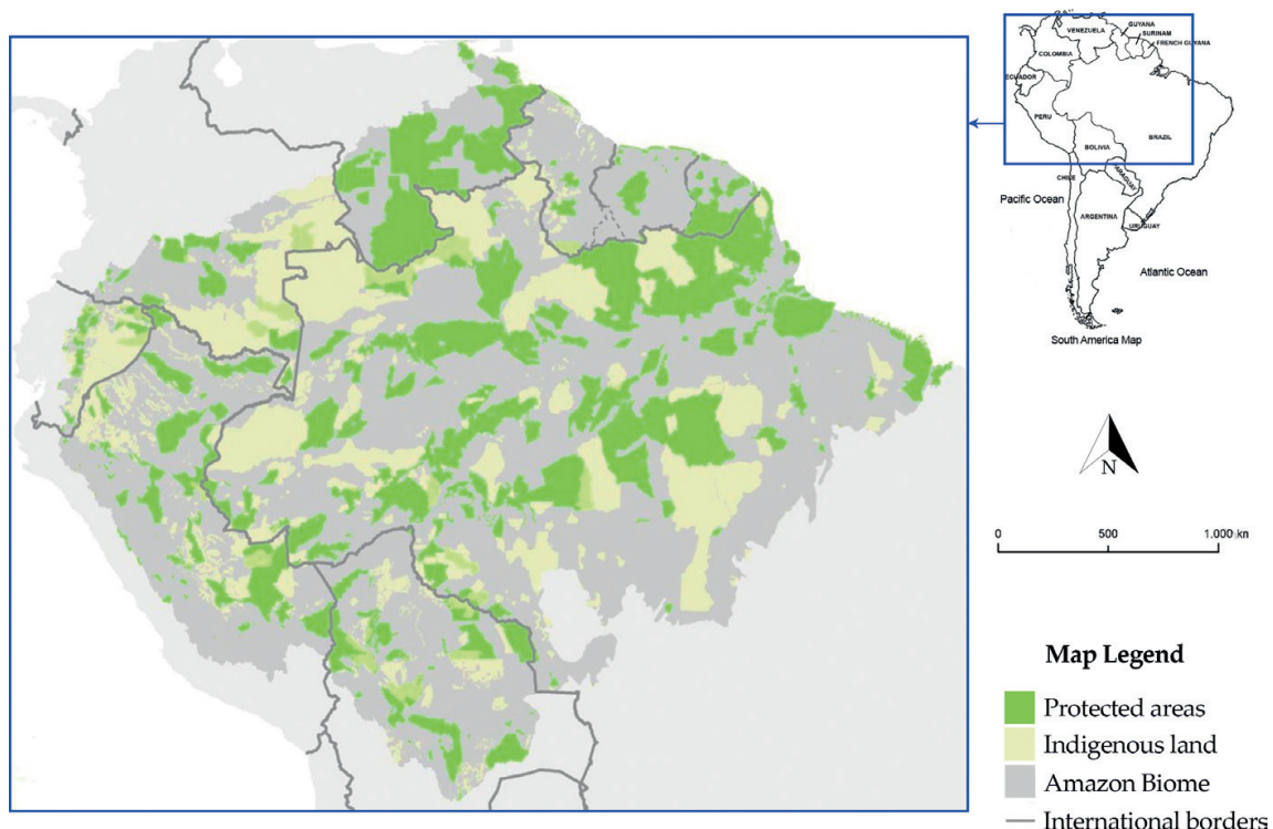
Figure 2. Protect areas in the Amazon basin. Source: Conservation International [8].
