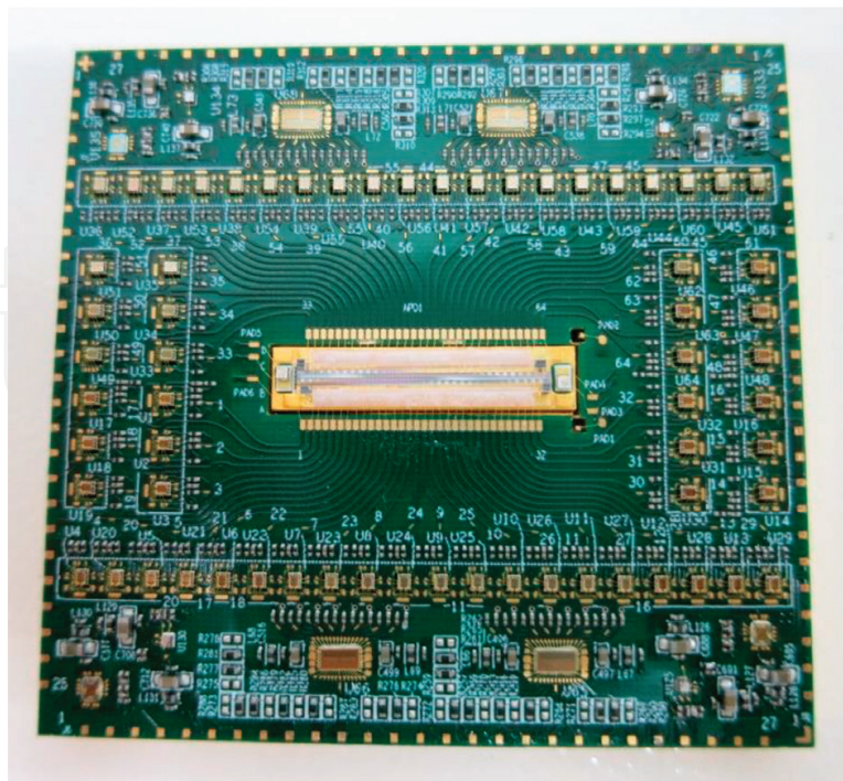
Figure 5. The device of 64 \times 1 linear-mode Si APD focal-plane array.
