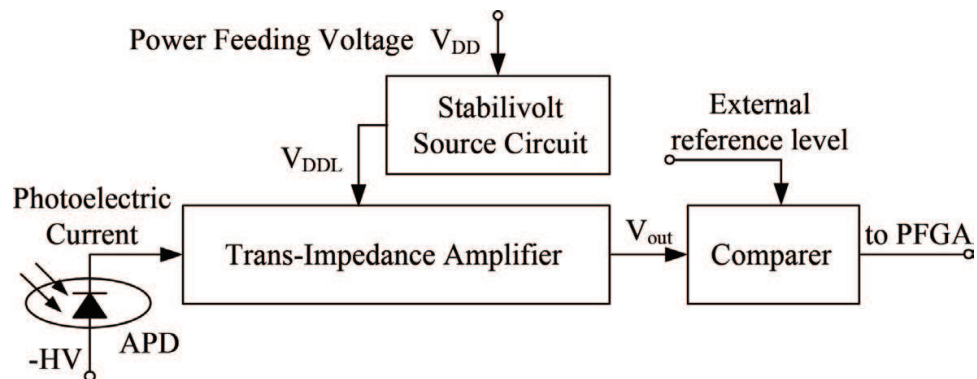
Figure 1. Schematic of the linear-mode Si APD.
