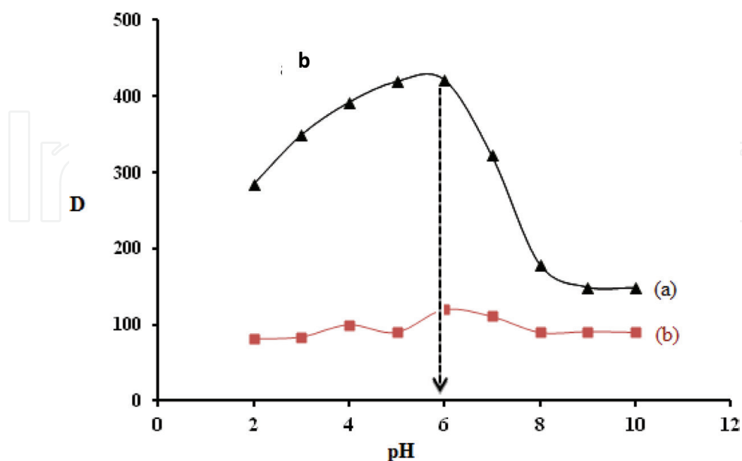
Figure 4. Plot of distribution ratio of mercury(II) ion uptake by TAR-treated PUFs (a) and unloaded PUFs (b) versus pH at 25^\circ\text{C} after 1-h shaking.
