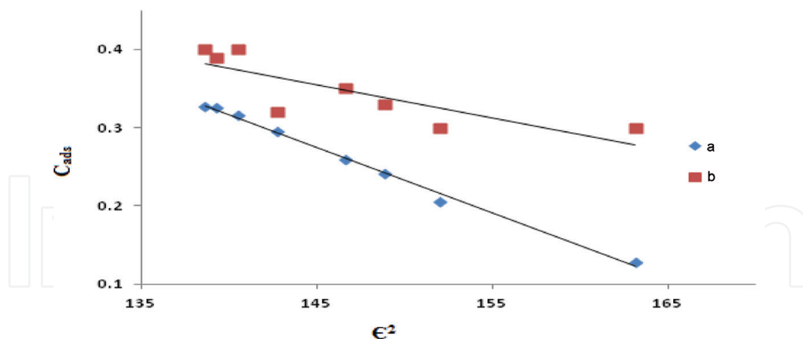
Figure 20. Dubinin-radushkevich (D-R) sorption isotherms of the mercury(II) ion uptake at optimal conditions by unloaded (a) and TAR-loaded PUFs sorbents (b) at 25°C after 1-h shaking.
