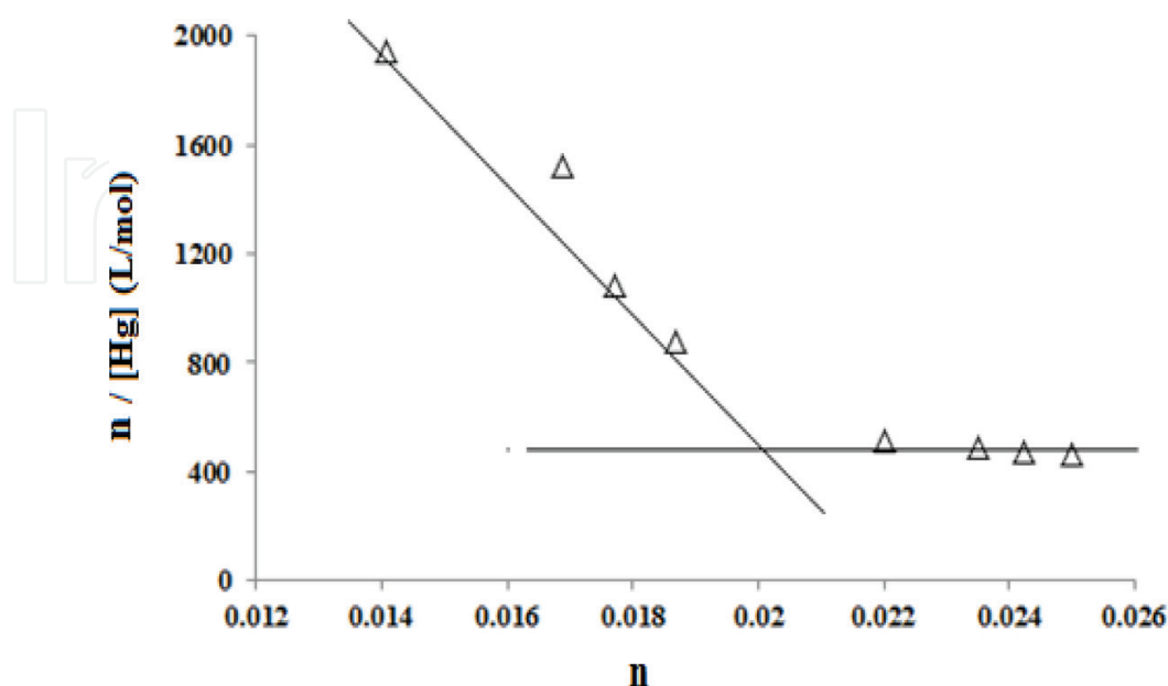
Figure 5. Scatchard plot of the sorption of mercury(II) ions from the aqueous media onto TAR-immobilized PUFs sorbents at 25°C after 1-h shaking.
