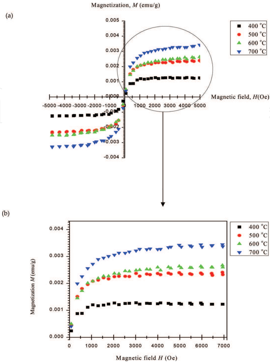
Figure 5. (a) Hysteresis loop of Ni 0.7 Zn 0.3 Fe 2 O 4 ferrite thin films and (b) first quadrant of the magnetic hysteresis loops of the samples. Magnetization at any given field increased with heat treatment temperature. Reproduced with permission from [21].
