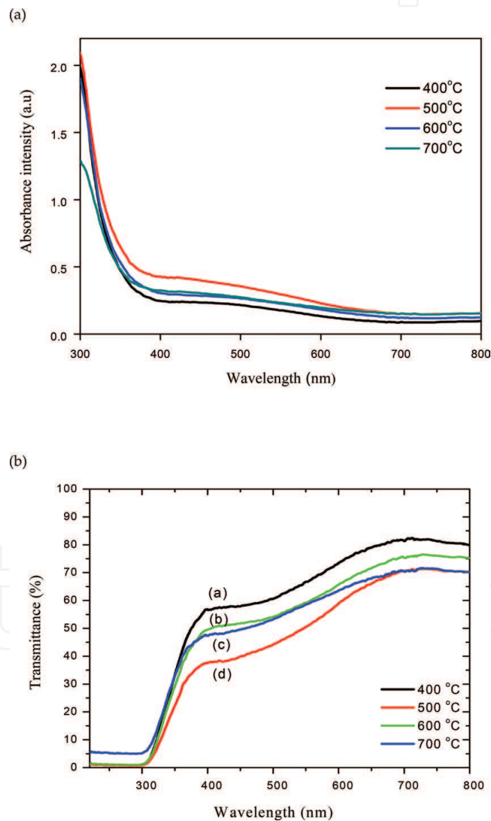
Figure 7. (a) Absorbance spectra of thin film at various annealed temperatures and (b) transmittance spectra of NiZn ferrite thin films.
