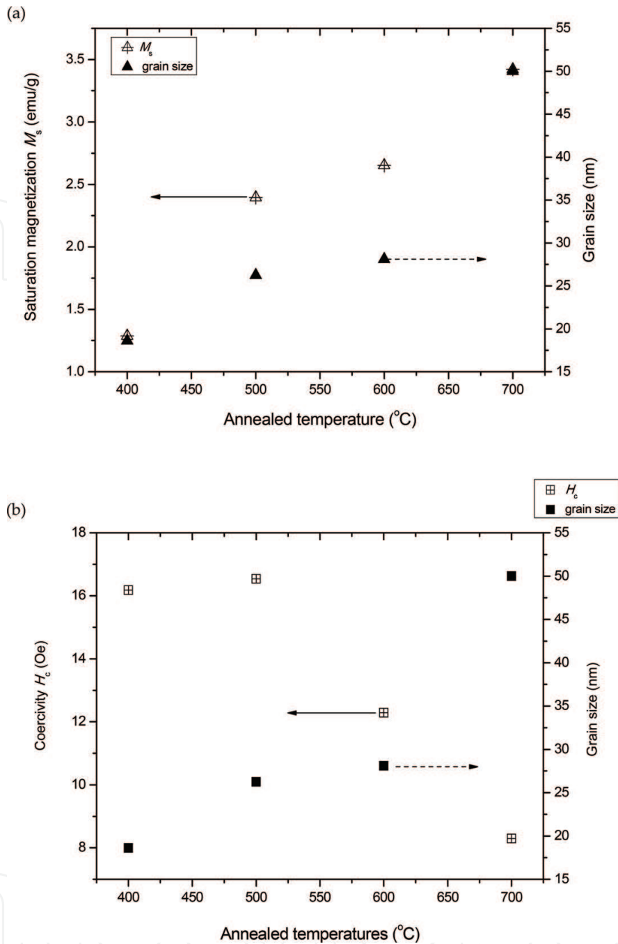
Figure 6. Comparison of the variation in (a) M_s and (b) H_c as a function of annealed temperatures of the \text{Ni}_{0.3}\text{Zn}_{0.7}\text{Fe}_2\text{O} nanoferrite thin films. Reproduced with permission from [21].
