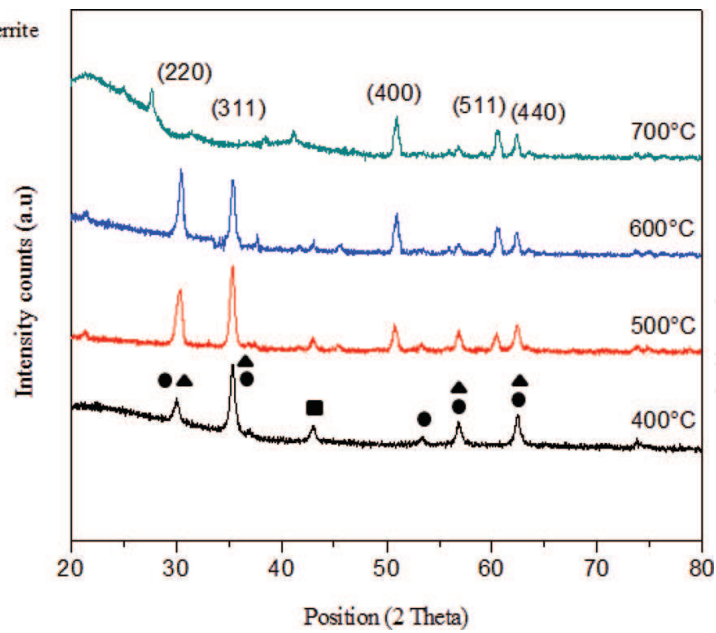
Figure 1. XRD pattern of air-annealed \text{Ni}_{0.3}\text{Zn}_{0.7}\text{Fe}_2\text{O}_4 ferrite thin films. Reproduced with permission from [21].
