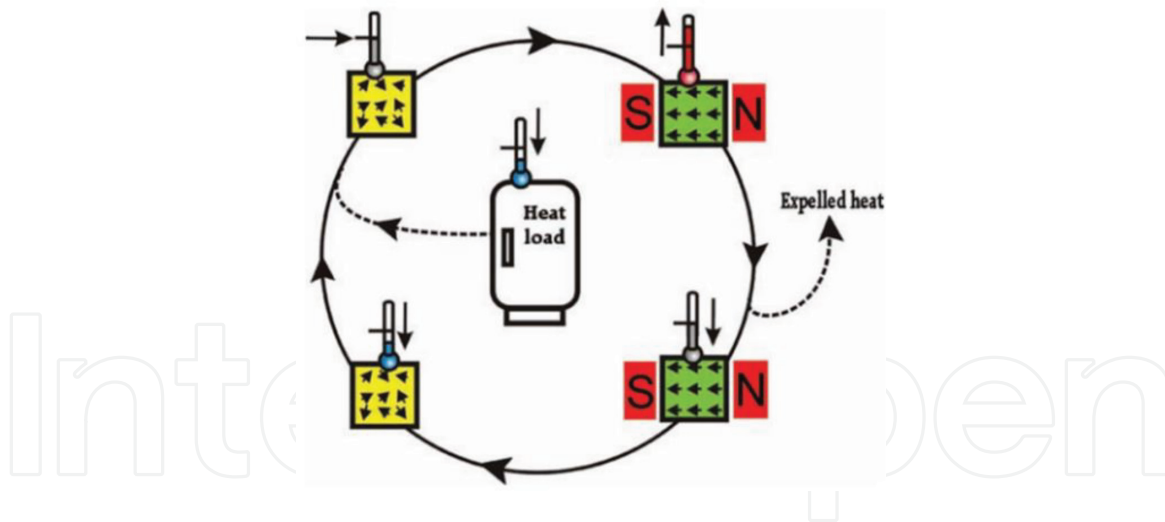
Figure 4. Schematic representation of a magnetic refrigeration cycle that transports heat from the heat load to the ambient environment. Yellow and green boxes depict materials in low and high magnetic fields, respectively. Reproduced with permission [20]. Copyright 2005, Institute of Physics.
