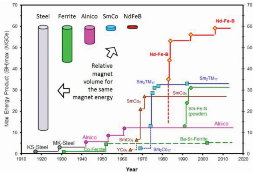
Figure 2. Development in the energy density (BH)_{max} at room temperature of hard magnetic materials in the twentieth century and presentation of different types of materials with comparable energy density. Reproduced with permission from [3].
