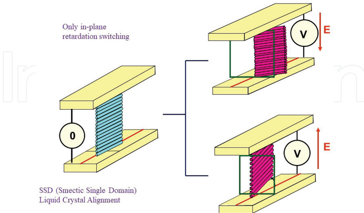
Figure 14 An overall concept of smectic single domain (SSD) liquid crystal molecular switching behavior. At the initial molecular alignment configuration, all of smectic liquid crystal molecules align uniformly forming like “liquid crystal wall”. When downward voltage is applied to the liquid crystal panel, the “liquid crystal wall” rotates clockwise direction. When upward voltage is applied, the “liquid crystal wall” rotates counter-clockwise direction.
