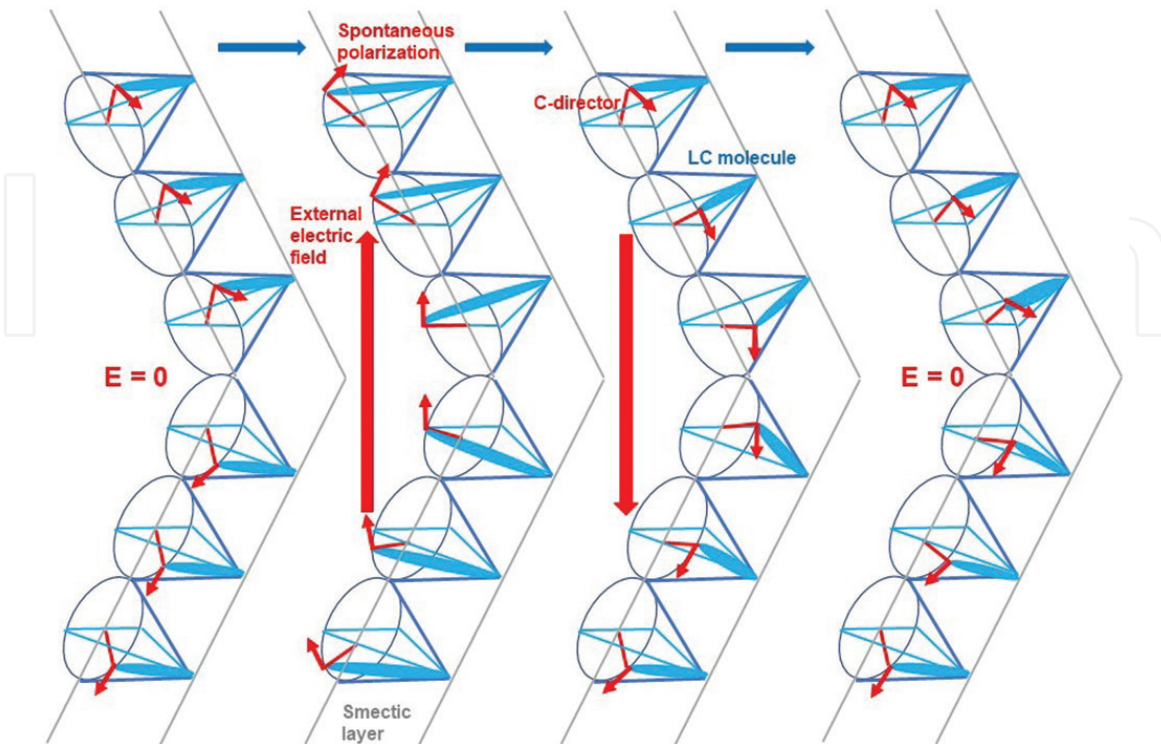
Figure 4 A non-reciprocal smectic layer switching of Chevron C1 uniform structure. Due to significant conflict in c-director packing at the kink area, repeating driving sometimes provides irreversible c-director packing after removing driving voltage. This results in instable electro-optic switching.
