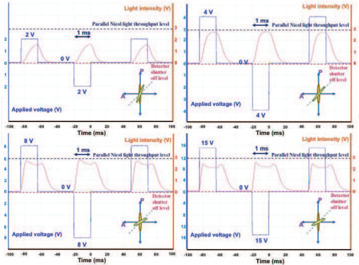
Figure 13 Light intensity profiles depending on applied electric field strength using the crossed Nicol optical set-up with 1 ms pulse voltage. Up to 4 V pulse voltage, light intensity gives almost maximum intensity. 8 V pulse voltage gives “bump” in light intensity during pulse voltage application, which strongly indicates over 45° optical axis rotation. Further increase in pulse voltage such as 15 V even gave lower reachable light intensity during pulse voltage application. This also indicates over 45° rotation under the premise of almost in-plane only retardation change.
