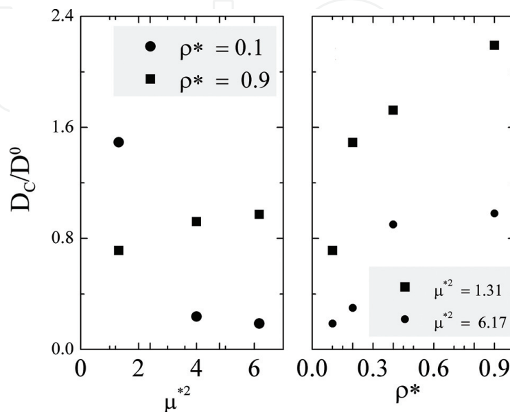
Figure 3. Calculated collective diffusion coefficient D_c normalized to the free particle diffusion constant at the hydrodynamic limit of low wavenumber k=0 . Notice that at high density, \rho^* = 0.9 , this property increases (left, black square symbol).
