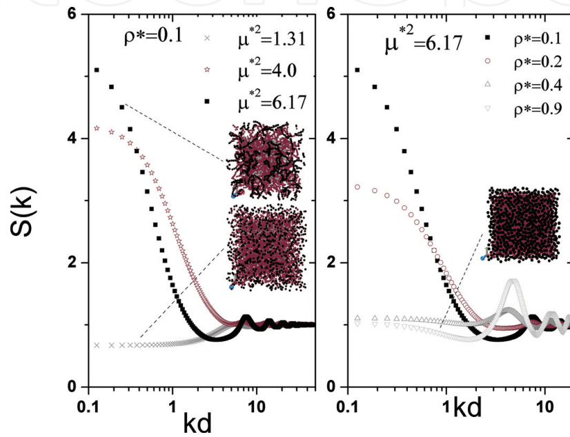
Figure 2. Simulation results of structure factor versus wave number. The contact values at k=0 yield the compressibility modulus. The material parameters of maghemite colloid were used [40]. At low densities and magnetic moment, there is liquid order. For higher dipole moments formation of chain appears.
