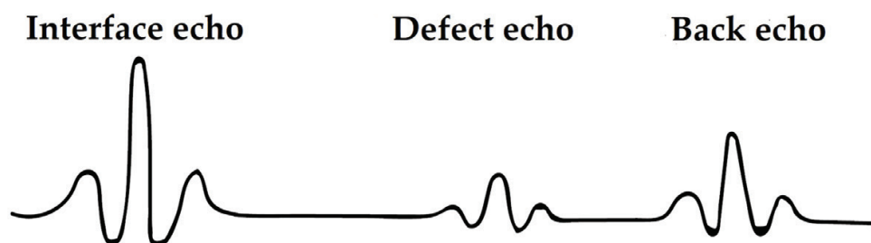
Figure 8. UT waveform generated during UT pulse-echo inspection of a defective part.
