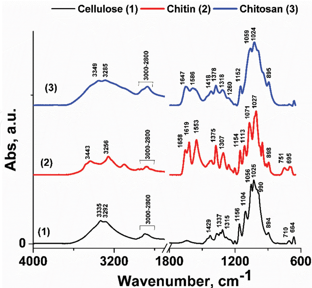
Figure 4. FTIR spectra of cellulose, chitin, and chitosan in the wavenumber region of 4000\text{--}600\text{ cm}^{-1} .
