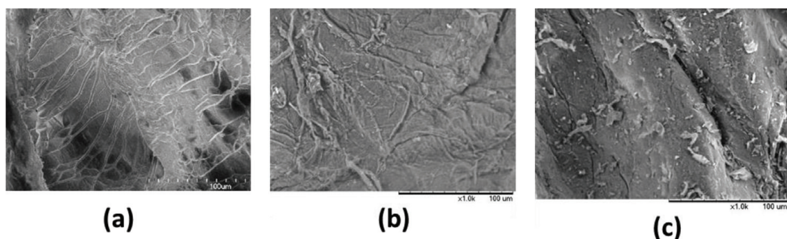
Figure 6. SEM images of (a) microcrystalline cellulose, (b) chitin and (c) chitosan at 100 μm magnification.
