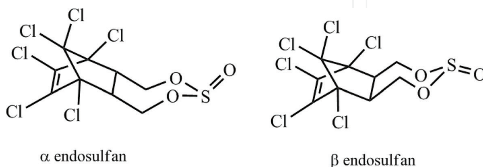
Figure 1. Structure of isomers \alpha and \beta endosulfan.
