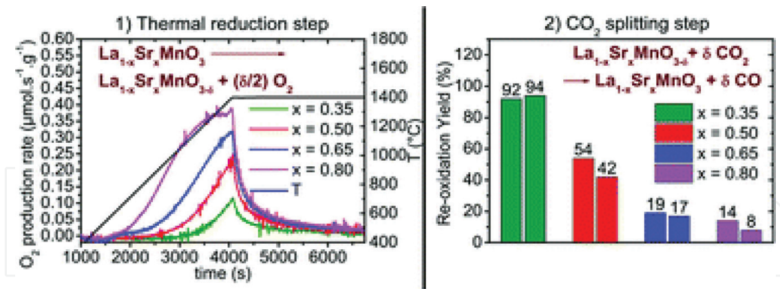
Figure 6. Solar-driven two-step thermochemical dissociation of \text{CO}_2 in \text{La}_{1-x}\text{Sr}_x\text{MnO}_{3-\delta} [67].
