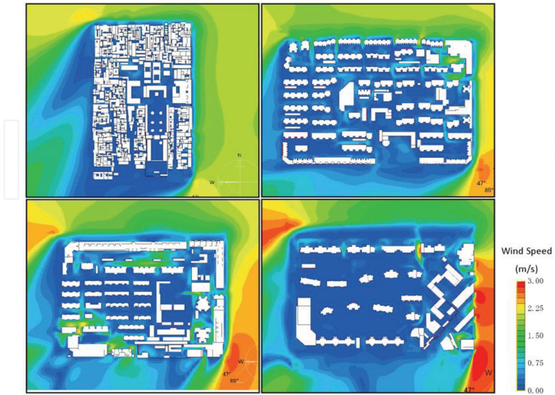
Figure 8. Wind speed distribution in four selected areas at 1.5 m height from the ground in summer (wind speed: 2 m/s; wind direction: EN).
