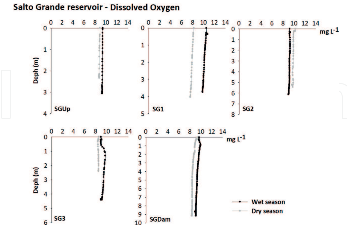
Figure 12. Dissolved oxygen profiles in Salto Grande reservoir sampling sites during wet and dry seasons.
