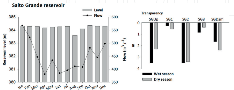
Figure 10. Variation of water level and flow (monthly averages) and transparency (wet and dry seasons) in Salto Grande reservoir.
