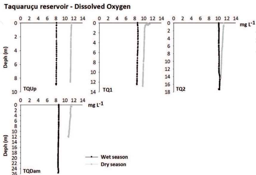
Figure 28. Dissolved oxygen profiles in Taquaruçu reservoir sampling sites during wet and dry seasons.
