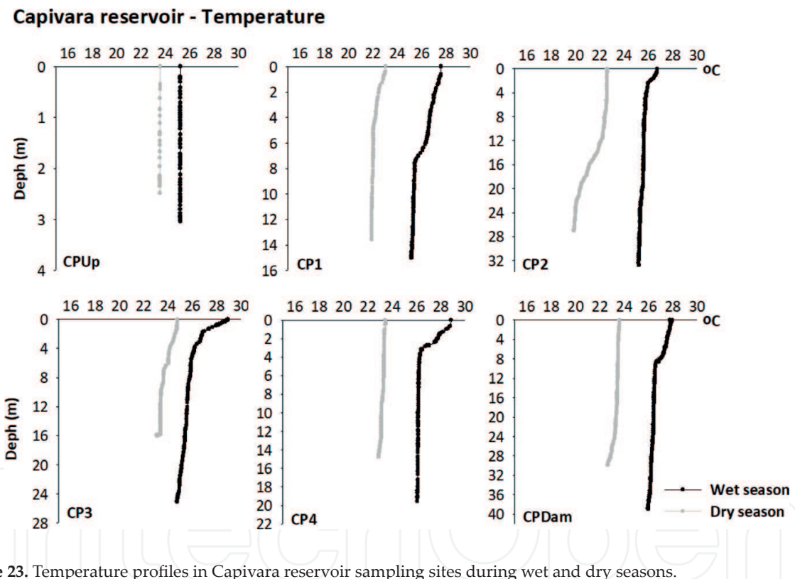
Figure 23. Temperature profiles in Capivara reservoir sampling sites during wet and dry seasons.
