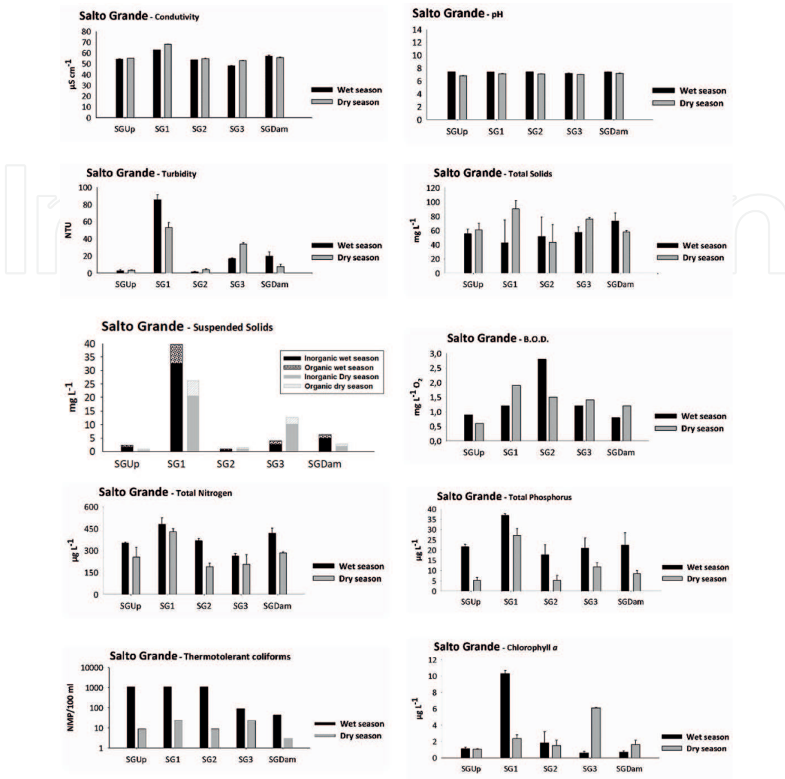
Figure 13. Mean values (+S.D.) of conductivity, pH, turbidity, total and suspended solids, biochemical oxygen demand, total nitrogen, total phosphorus, thermotolerant coliforms and chlorophyll a in Salto Grande reservoir sampling sites in the 2011 wet and dry seasons.
