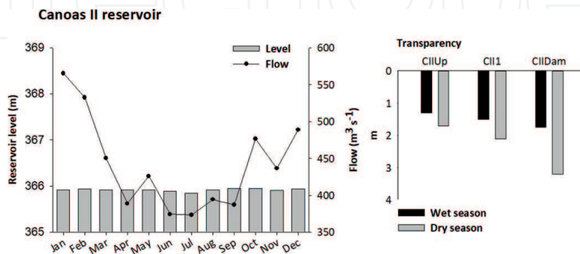
Figure 14. Variation of water level and flow (monthly averages) and transparency (wet and dry seasons) in Canoas II reservoir.
