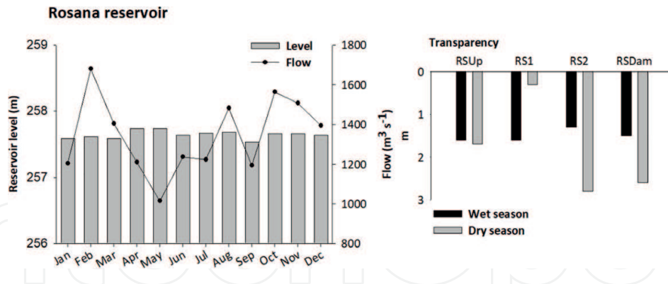
Figure 30. Variation of water level and flow (monthly averages) and transparency (wet and dry seasons) in Rosana reservoir.
