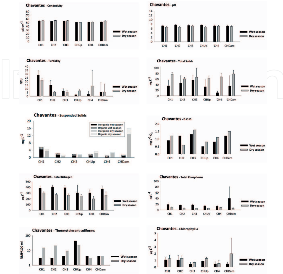
Figure 9. Mean values (+S.D.) of conductivity, pH, turbidity, total and suspended solids, biochemical oxygen demand, total nitrogen, total phosphorus, thermotolerant coliforms and chlorophyll a in Chavantes reservoir sampling sites during wet and dry seasons.
