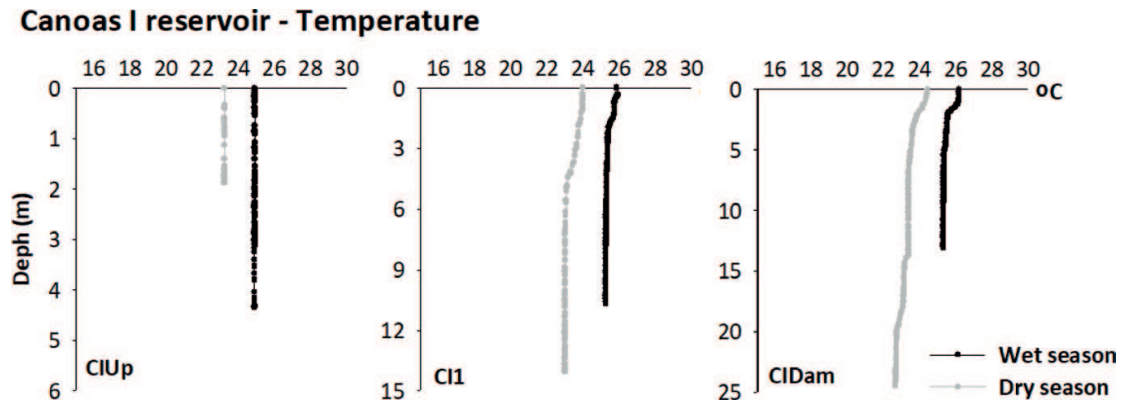
Figure 19. Temperature profiles in Canoas I reservoir sampling sites during wet and dry seasons.
