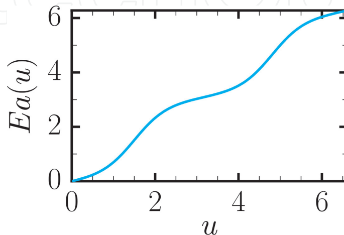
Figure 6. Plot of Ea(u) for A = 0.1 , B = 0.9 , and \alpha = 1.2 .
