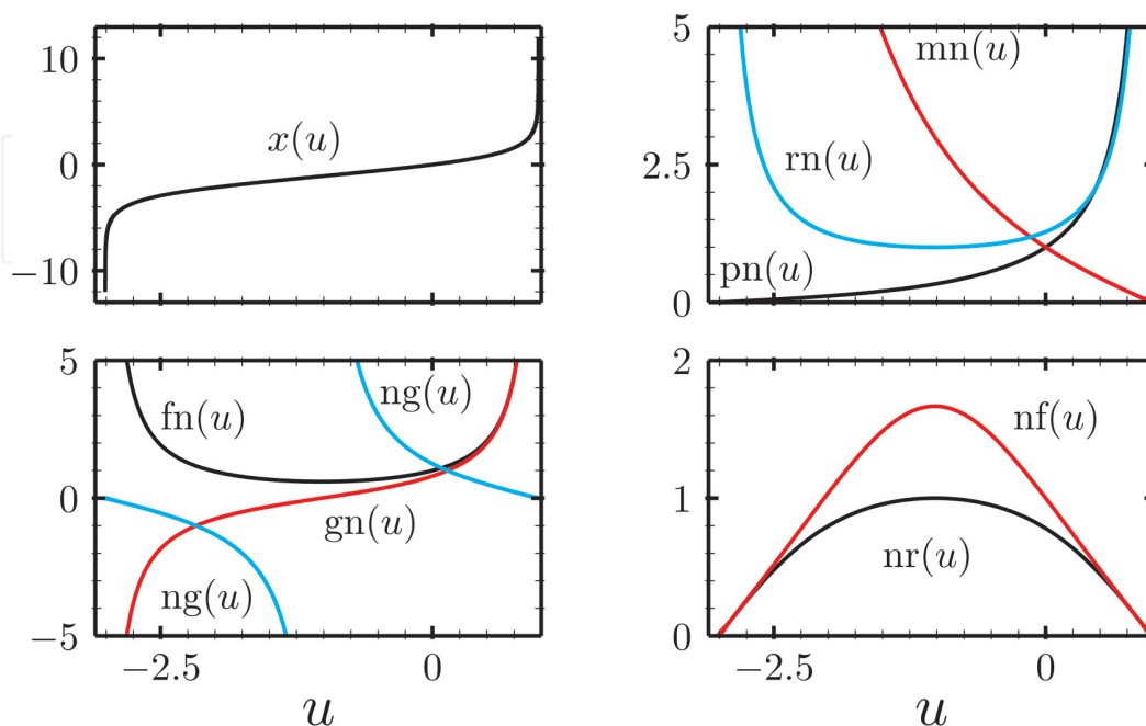
Figure 7. Nonlinear exponential-like functions for m = 1 , a = 0.1 , and b = 0.9 .
