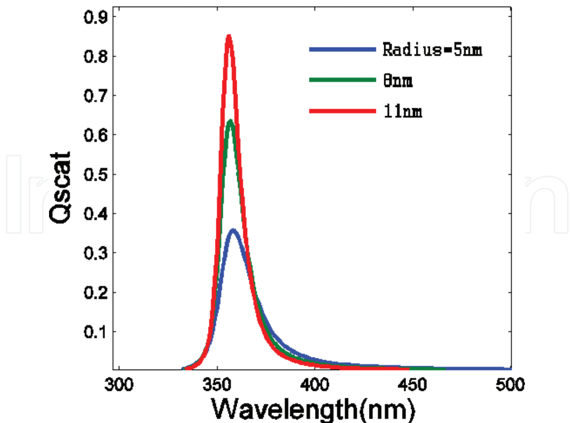
Figure 2. Wavelength dependent scattering cross section of silver metal nanoparticle of three different radii.
