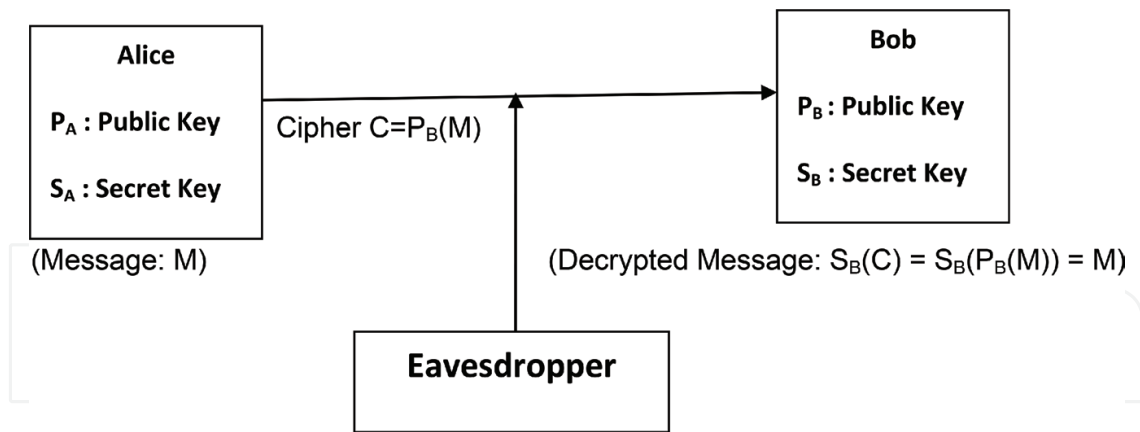
Figure 2. Public-key cryptosystem.
