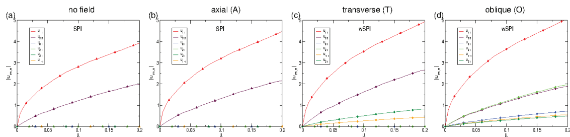
Figure 5. Bifurcation diagrams of SPI and wSPI, respectively, in different magnetic fields: (a) no field (N), (b) axial (A), (c) transverse (T), and (d) oblique (O). Moduli |u_{m,n}| (18) of the radial flow field amplitudes at mid gap are shown versus the relative distance \mu = \text{Re}_1/\text{Re}_{1,onset} - 1 from the onset of the respective vortex flow. Further parameters are: \text{Re}_2 = -150, \beta = 0.5, k = 3.927 (cf. Figure 2 ).
