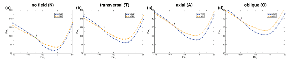
Figure 8. Bifurcation curves for the onset of (w)TVF (blue) and (w)SPI (orange) in Re_2 - Re_1 diagram under (a) no magnetic field (N) ( s_x = 0, s_z = 0 ), (b) an applied transversal field (T) ( s_x \neq 0, s_z = 0 ), (c) an applied axial field (A) ( s_x = 0, s_z \neq 0 ), and (d) an applied oblique field (O) ( s_x \neq 0, s_z \neq 0 ). Simulation results of full nonlinear Eqs. (11) consider short periodic TCS with k = 3.927 (cf. [6, 28]).
