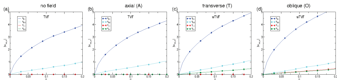
Figure 4. Bifurcation diagrams of TVF and wTVF, respectively, in different magnetic fields: (a) no field ( N ), (b) axial ( A ), (c) transverse ( T ), and (d) oblique ( O ). Moduli |u_{m,n}| (18) of the radial flow field amplitudes at mid gap are shown versus the relative distance \mu = \text{Re}_1/\text{Re}_{1,c} - 1 from the onset of the respective vortex flow. Further parameters are: \text{Re}_2 = 0, \beta = 0.5, k = 3.927 (cf. Figure 2 ).
