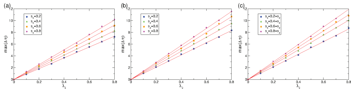
Figure 14. Supercritical ( w )TVF solution at Re_1 = 100 , Re_2 = 0 . Variation of vorticity maxima \max(\eta) = \eta(\lambda_2) - \eta(\lambda_2 = 0) for (a) transversal (T), (b) axial (A) and (c) oblique (O) magnetic field (strength as indicated). Lines are linear fits.
