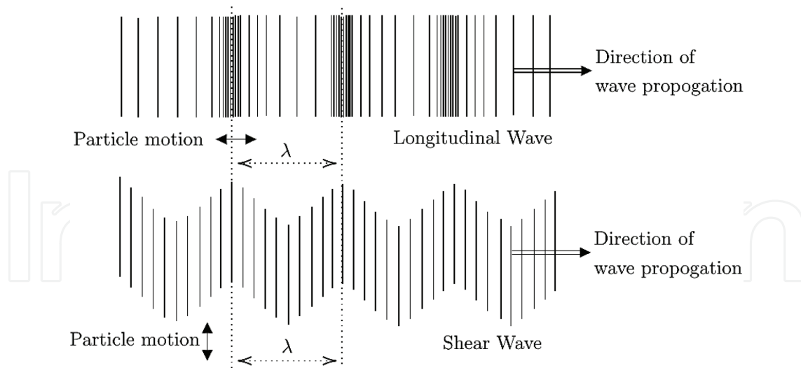
Figure 2. Illustration of particle motion in the two bulk wave modes: longitudinal and shear.
