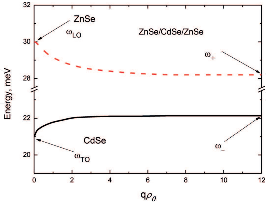
Figure 1 . Wave vector dependencies of interface optical phonon energies for ZnSe/CdSe/ZnSe quantum wire; m = 0 .
