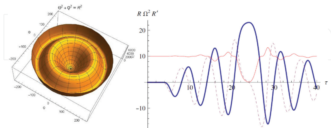
Figure 4. Two-dimensional potential with two minima which correspond to destroy DNA schemes represented in Figures 1 and 2 . First minimum corresponds to nondimmer DNA and second minimum to the dimerization of DNA under the UV-C radiation. In the right hand, the transfer of DNA from first minimum to the second minimum is plotted. The thick line represents the behavior of R(t) , the red line to nonlinear oscillatory frequency in the relative units \Omega^2/\Omega_0 and \tau = t/\Omega_0 .
