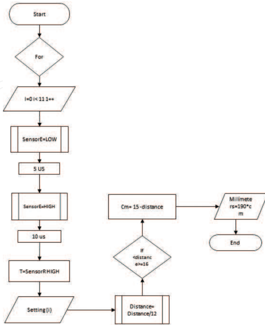
Figure 11. Block diagram of programming using Arduino.
