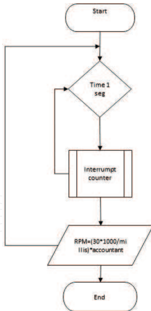
Figure 9. Block diagram of the program to measure rpm.
