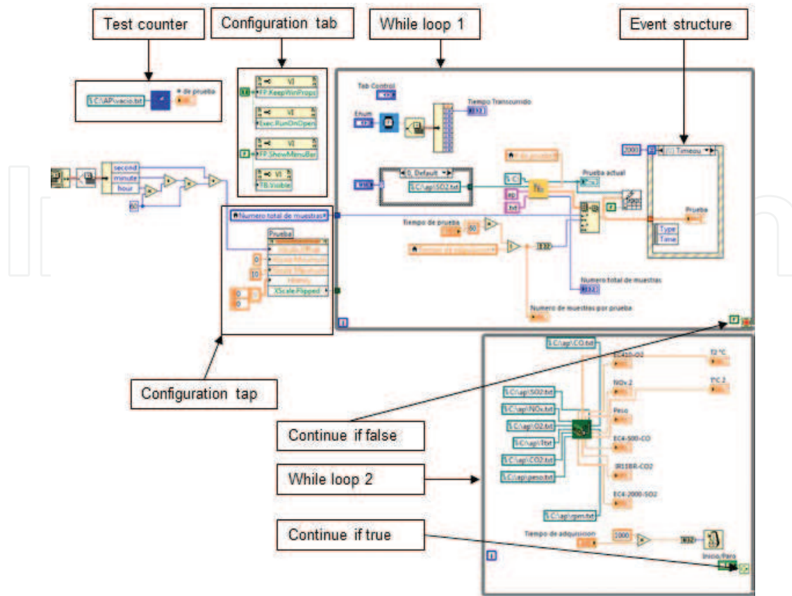
Figure 7. Block programming.
