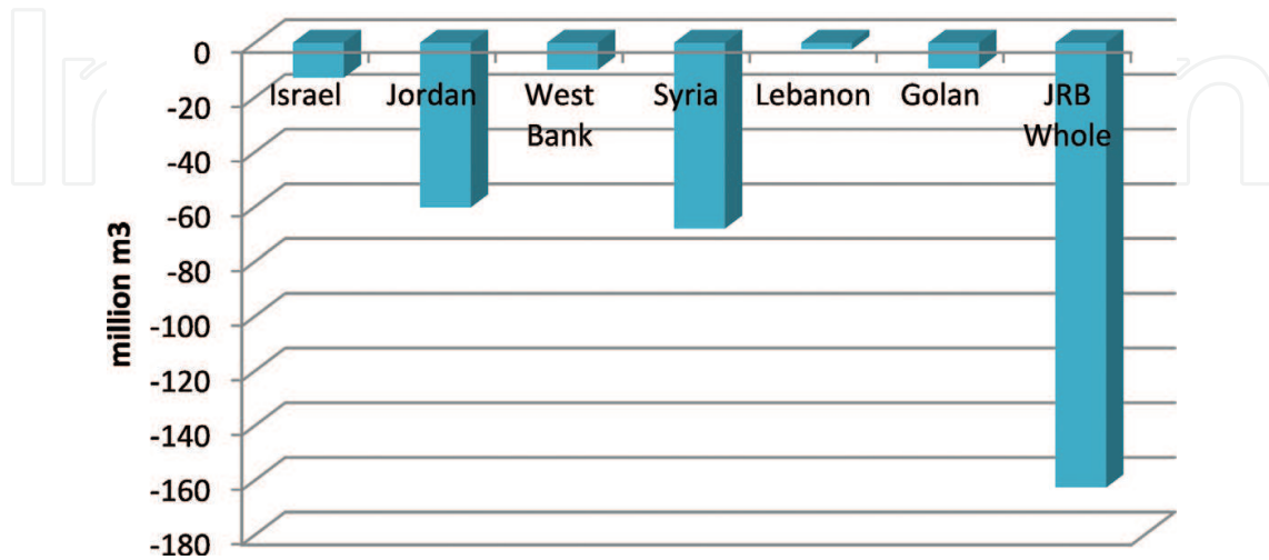
Figure 6. Impact of climate change on run-off.
