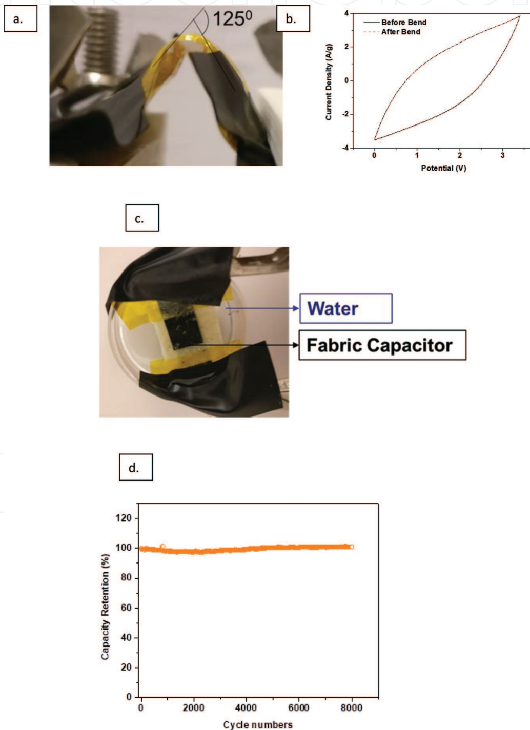
Figure 8. (a) Picture of the degree of bending during each cycle of the stress test; (b) cyclic voltammeter curve of the device before and after bending; (c) picture of the water bath immersion tests; and (d) cycling curve of the device at 2 A/g current density.
