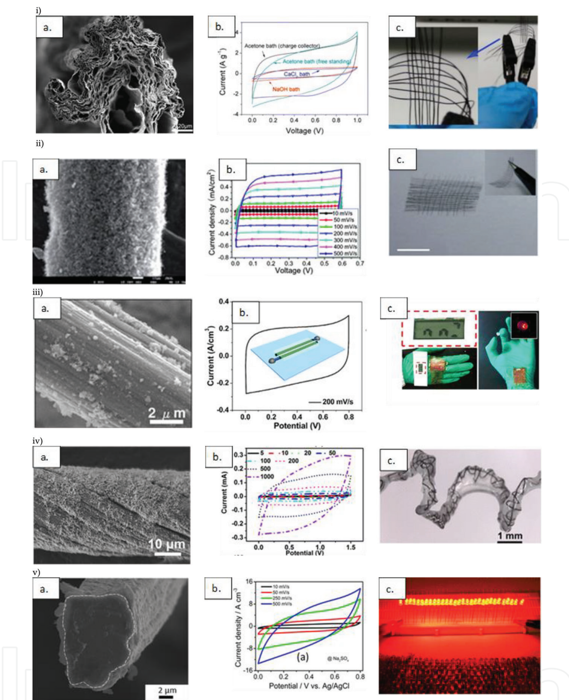
Figure 5. (a) SEM image of electrode base material; (b) cyclic voltammetry graph of the working device; (c) picture of full device. (i) RGO fiber reprinted with permission from [49]. Copyright 2014 American Chemical Society. (ii) CNT-graphene fiber reproduced from [48] with permission from Royal Society of Chemistry. (iii) Carbon fiber coated with manganese oxide reprinted with permission from [50]. Copyright 2012 American Chemical Society. (iv) CNT fiber coated with manganese oxide reprinted with permission from [51]. Copyright 2015 American Chemical Society. (v) GO-active material coated stainless steel fiber reprinted with permission from [52]. Copyright 2015 American Chemical Society.
