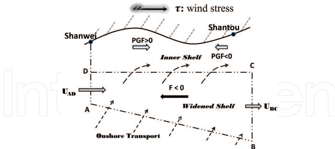
Figure 7. Schematic picture showing the wind-driven upwelling processes and forcing mechanism over the middle and inner shelves of a widened shelf. Redrawn from Gan et al. [91]. PGF denotes pressure gradient force; U_{AD} and U_{BC} are mean velocities normal to the two streamlines AD and BC, respectively. The line AD is at the head of the widened shelf (near Shanwei) and BC, downstream of it (near Shantou).
