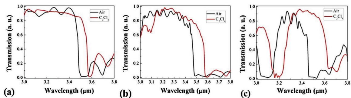
Figure 8. Simulated transmission with air-clad and C_2Cl_4 -clad conditions for (a) conventional PCW, (b) holey PCW, and (c) slotted PCW [45].
