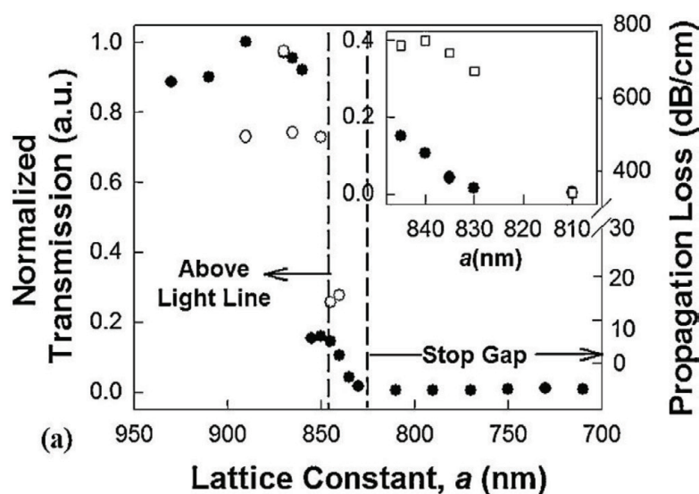
Figure 5. Lattice constant dependent transmission and propagating loss [45].
