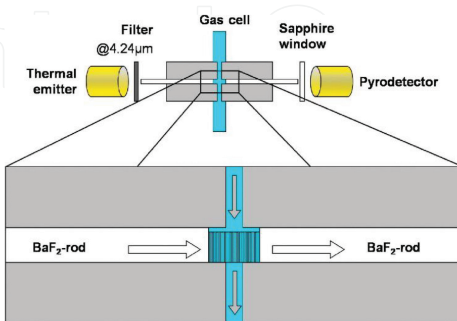
Figure 2. Schematic design used for gas absorption measurements [35].
