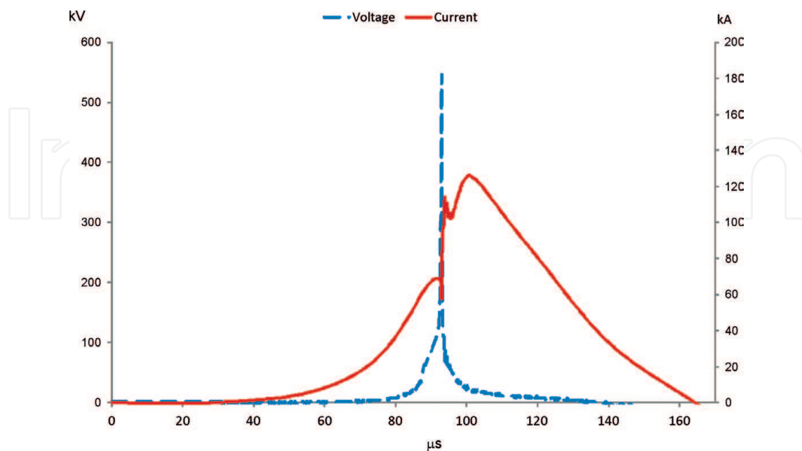
Figure 13. Experimentally obtained impulse current and voltage at the load (EEC).
