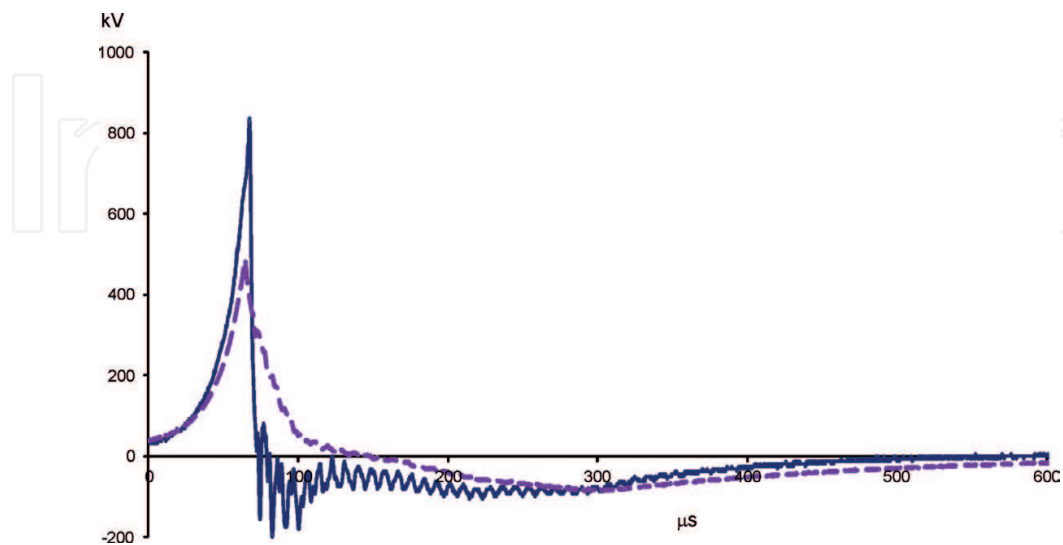
Figure 7. Voltage at the MTC EMG output from the voltage divider no. 1 and on the active load from the voltage divider no. 2.
