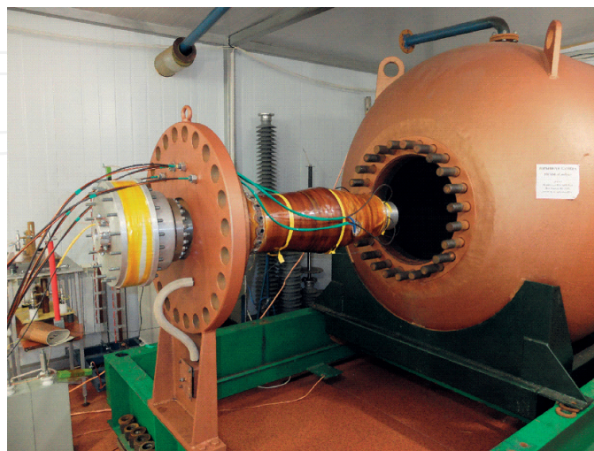
Figure 11. EMG assembly, before installation in the explosion protection chamber.
