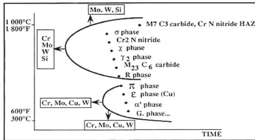
Figure 1. A schematic TTT curve for formation of precipitates in DSS and the effects of alloying elements in the temperature ranges of formation for various precipitates [10].
