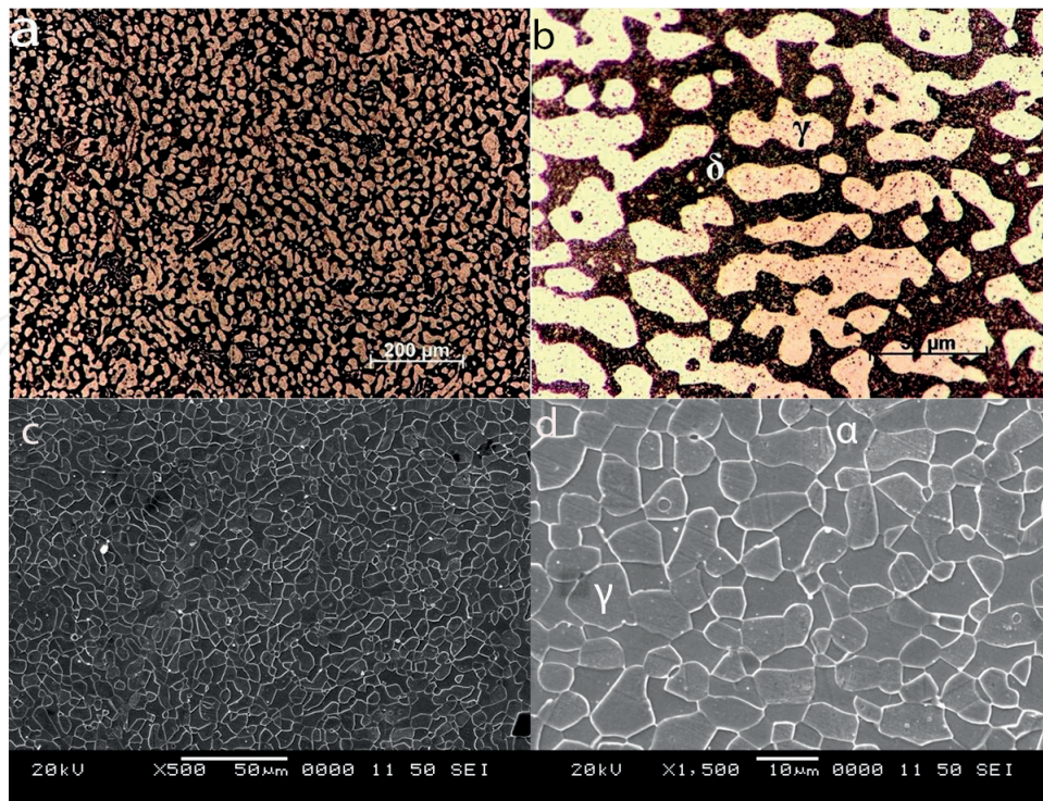
Figure 3. Microstructure of S2205 after solution heat treatment (a) OM image of distribution of austenite grains in the ferrite matrix (magnification: 100×). (b) OM image of phase morphology (magnification: 500×).
