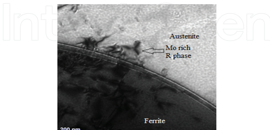
Figure 6. HR-TEM image of 60 min reversion heat treated sample showing clear austenite phase and ferrite phase with R-phase.
