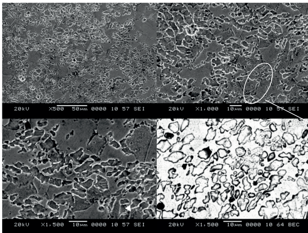
Figure 2. Microstructure of as received S2205 duplex stainless steel sample (Etchant:Beraha's tint etch).
