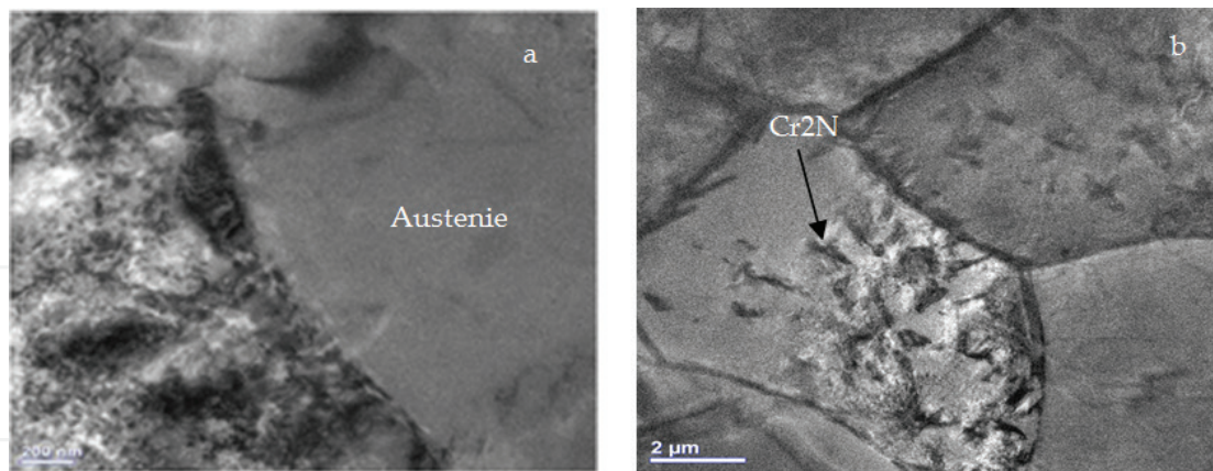
Figure 5. HR-TEM image of 1000 h aged sample showing (a) the mottled contrast ferrite region and precipitate free austenitic phase. (b) the morphology of Cr 2 N precipitates in ferrite matrix.
