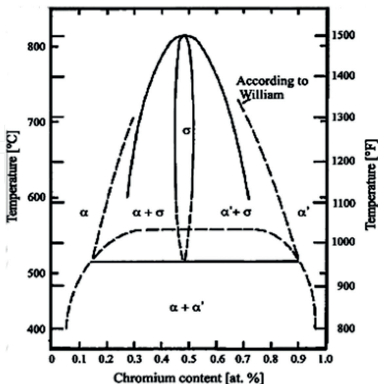
Figure 4. Phase diagram of the iron-chromium binary system.
