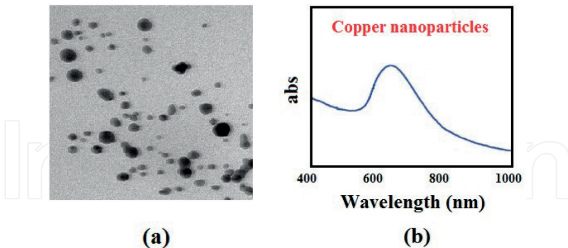
Figure 4. (a) TEM image of copper nanoparticle in oil and (b) UV-visible spectrum of copper nanoparticles produced using laser ablation.
