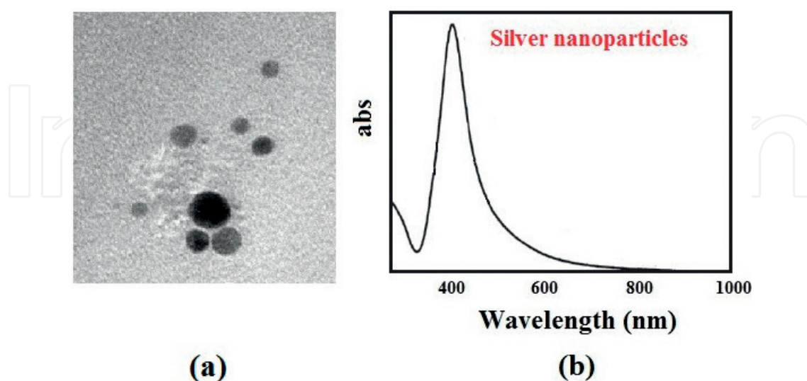
Figure 2. (a) TEM image of silver nanoparticle in oil and (b) UV-visible spectrum of silver nanoparticles produced using laser ablation.
