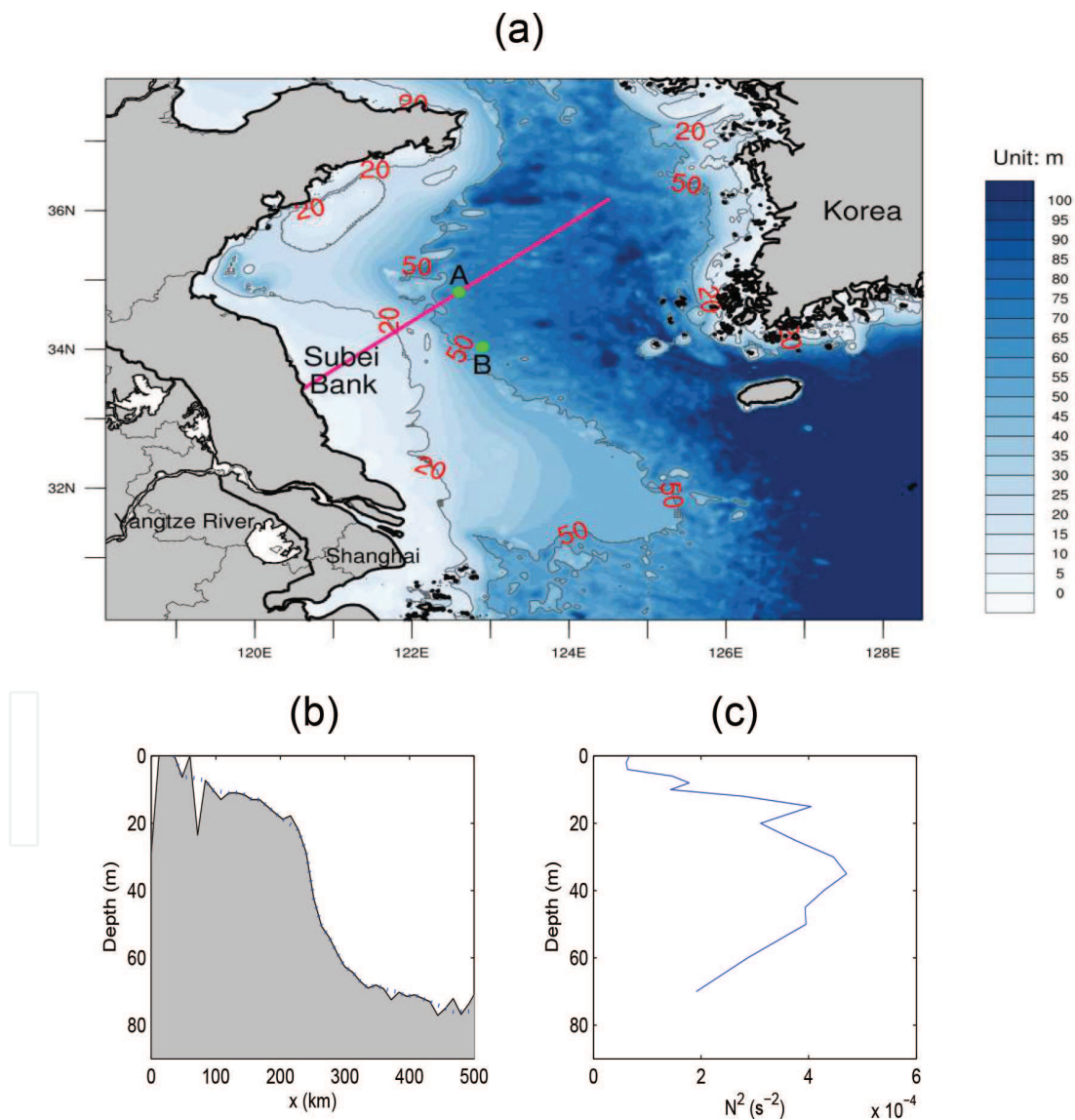
Figure 1. (a) Bathymetry of the Yellow Sea. Abutted to the left is China, while on its right lies Korea. The solid line across Subei Bank marks the cross-section which we will study. Also marked are the points A and B where time series will be extracted from the HYbrid Coordinate Ocean Model (HYCOM) dataset for analysis. (b) The topography along the section marked in (a). (c) A profile of the buoyancy frequency squared N^2 (for 1995).
