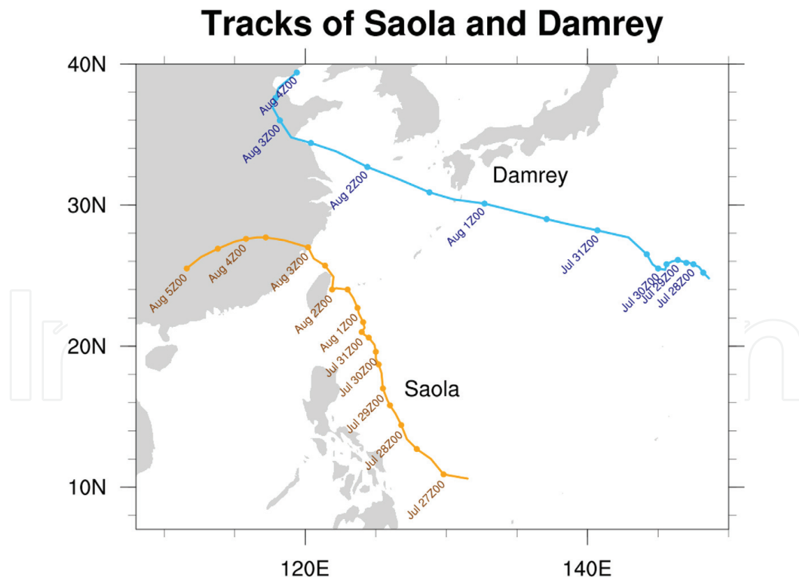
Figure 1. The paths of the twin typhoon Damrey and Saola (data courtesy of China Meteorological Administration).
