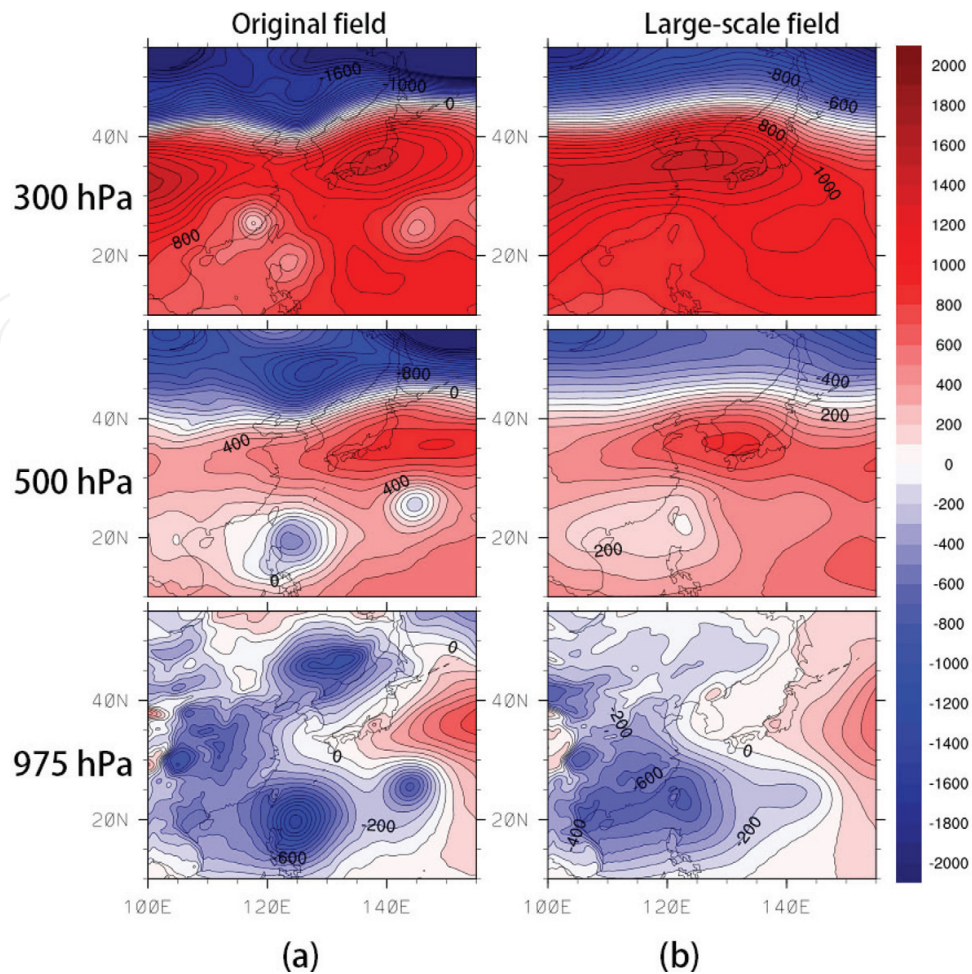
Figure 3. (a) The original geopotential ( m^2 \cdot s^{-2} ) and (b) its reconstruction on the large-scale window ( m^2 \cdot s^{-2} ) on July 30, 2012, at 975, 500, and 300 hPa.
