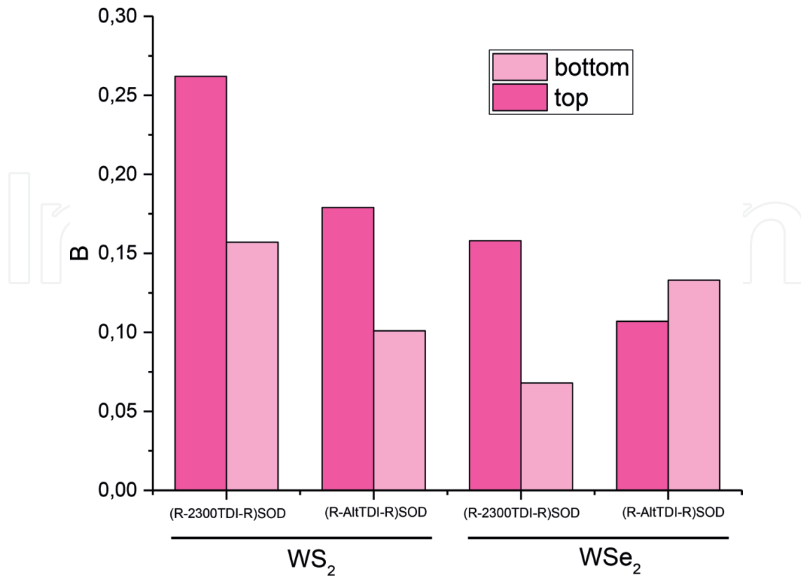
Figure 7. Friction coefficients of coPUIs based on (R-2300TDI-R)SOD (50) and (R-AltTDI-R)SOD (45) matrices modified by WS 2 and WSe 2 nanoparticles, determined by AFM method in the contact mode on one field.
