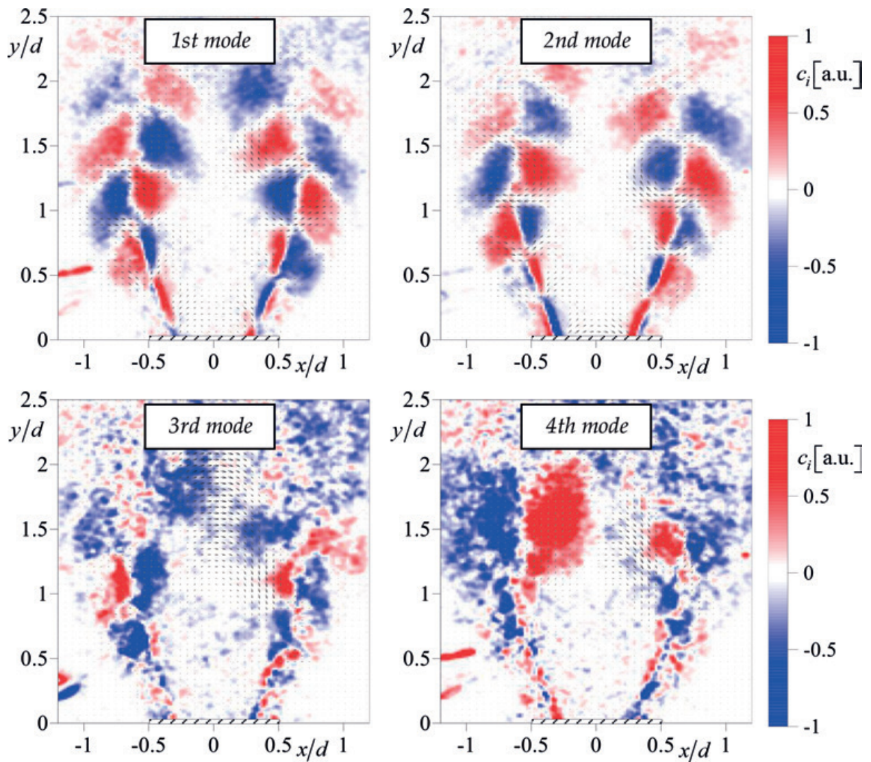
Figure 13. First four POD modes of the velocity fluctuations and conditionally sampled HCHO PLIF fluctuations for a high-swirl fuel-lean flame ( S = 1.0 , \varphi = 0.7 ).
