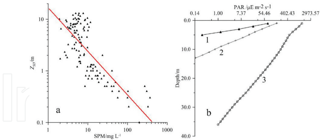
Figure 17. (a) Relation between SPM and Secchi disk depth ( Z_{sd} ), as well as least square regression line (red), for the southwestern Yellow Sea during spring 2012. (b) Vertical profiles of the PAR observed in the southwestern Yellow Sea during spring 2012.
