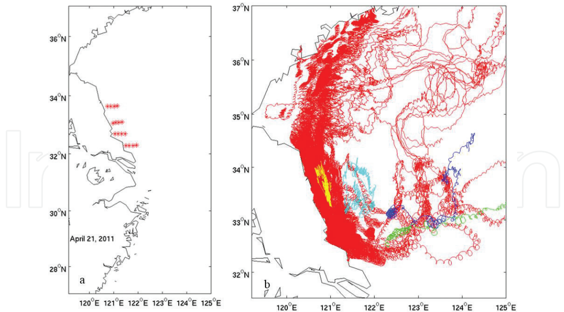
Figure 9. (a) Released locations for all particles, and (b) trajectories of all neutral particles released in the Subei area in 2011 (red) and satellite-tracked Argos drifters (other colors) at the same time.
