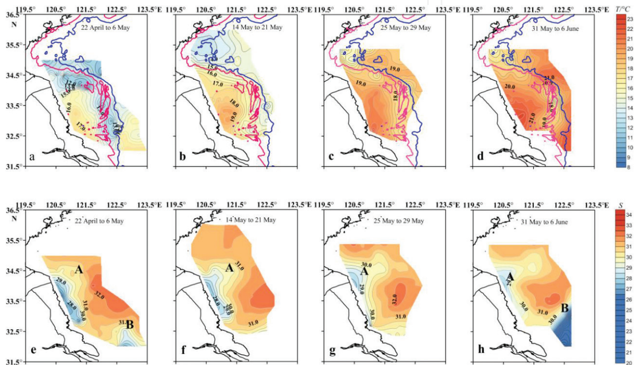
Figure 15. Distribution patterns of surface temperature ( ^{\circ}\text{C} , upper panels) and salinity (lower panels) from April 22 to may 6 (a, e), from may 14 to may 21 (b, f), from may 25 to may 29 (c, g), and from may 31 to June 6 (d, h) in 2012. The red and blue curves are the 20- and 30-m isobaths, respectively.
