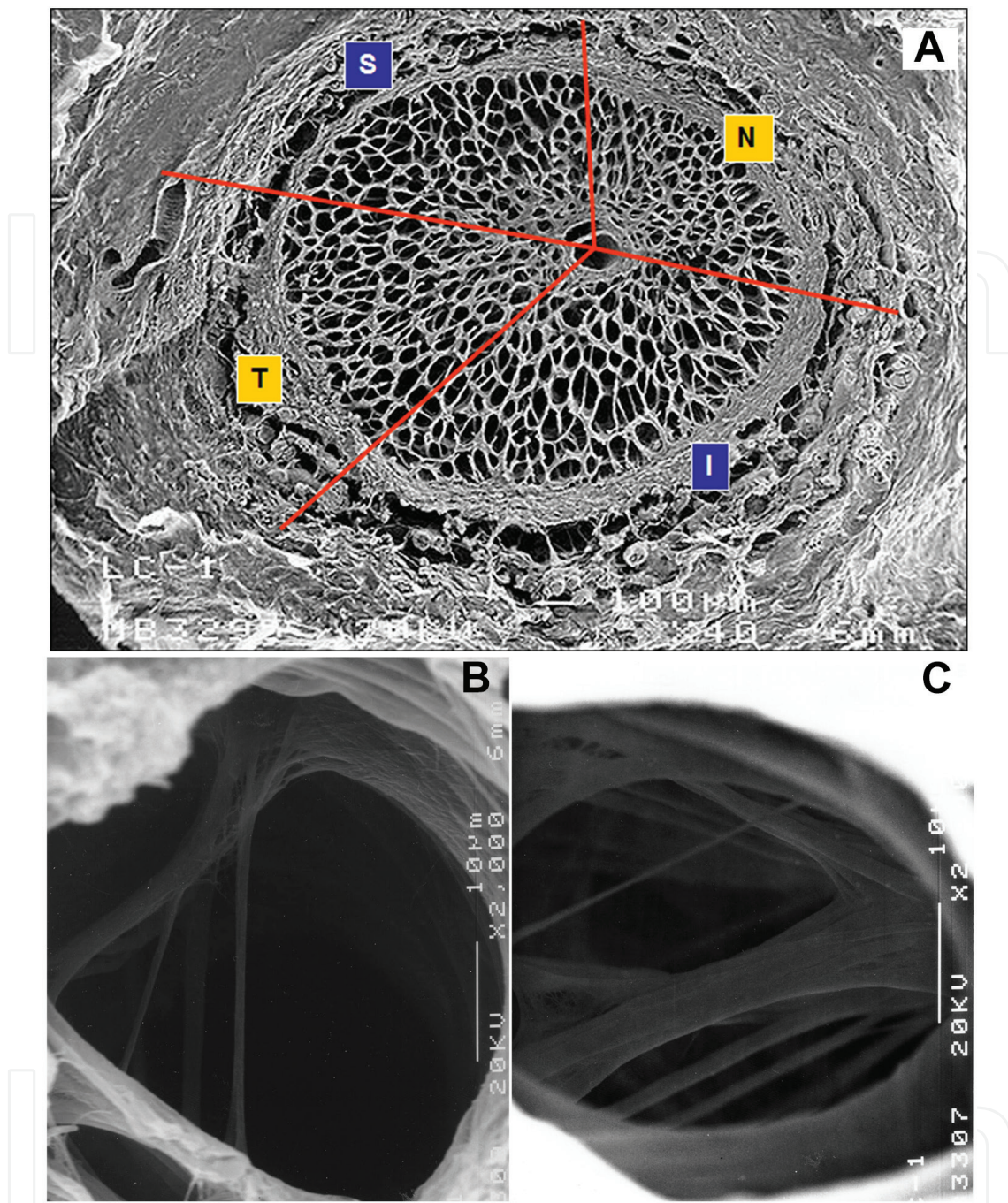
Figure 6. (A) Laminar region of the optic nerve head: Superior (S), nasal (N), inferior (I) and temporal (T) sectors. (B, C) detail of the cribriform pores: (B) nasal cribriform pore and (C) inferotemporal cribriform pore. (A–C) scanning electron microscopy with nervous tissue digestion by trypsin. (A: modified with permission from Ramírez et al. [181]).
