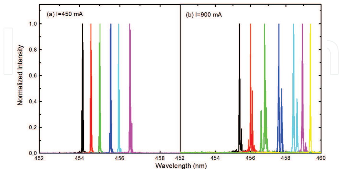
Figure 4. Optical spectra of the output beam from the ECDL system with (a) a holographic grating at an injected current of 0.45 A and (b) a ruled grating at an injected current of 0.9 A.
