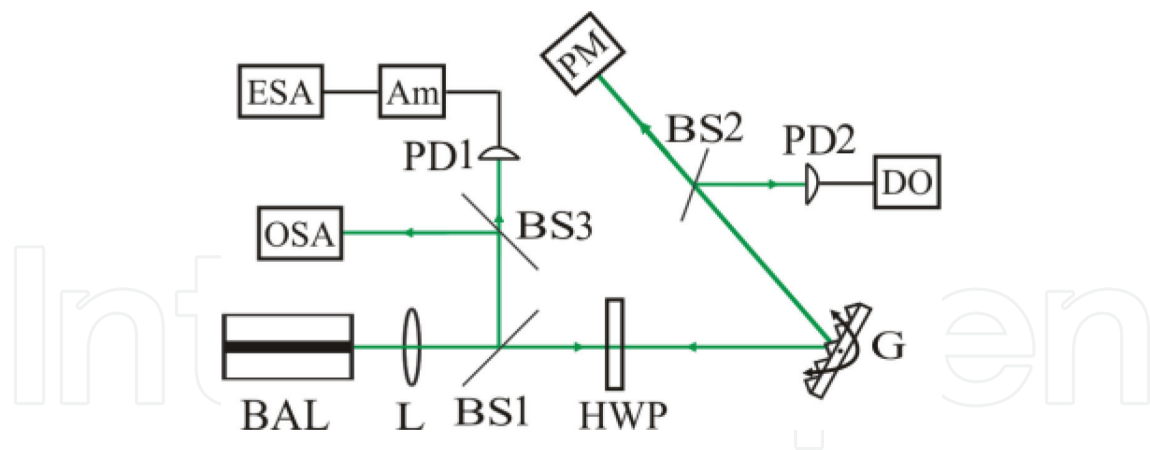
Figure 1. Experimental setup of the ECDL system. BAL, broad-area diode laser; L, lens; BS1, BS2 and BS3, beam splitter; HWP, half-wave plate; G, bulk grating; PD1 and PD2, photodiode; DO, digital oscilloscope; OSA, optical spectrum analyzer; Am, amplifier; ESA, electrical spectrum analyzer; PM, power meter.
