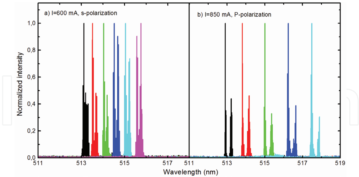
Figure 7. Optical spectra of the green ECDL system operates in (a) s -polarized mode and (b) p -polarized mode. The output power is around 290 mW for both operation modes.
